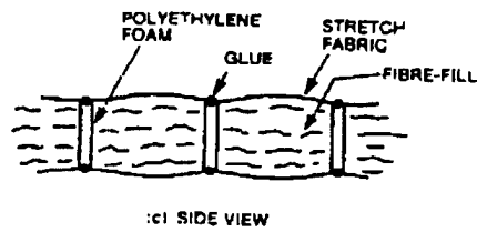
Fig. 3. The design of the sleeping bag and built-in pad.
