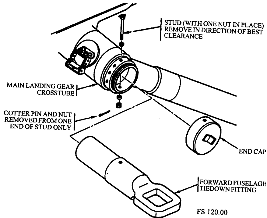
DETAIL A
