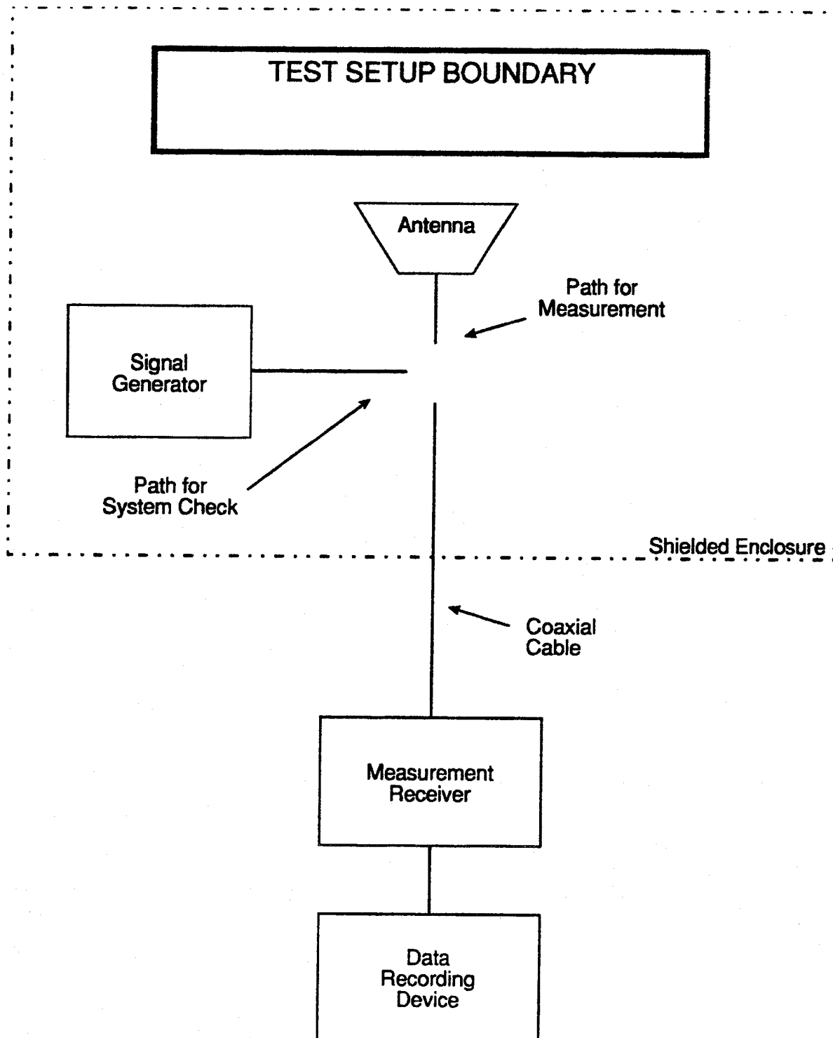
FIGURE RE102-1. Basic test setup.
