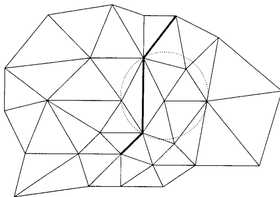
Figure 5: Illustration of constrained Delaunay triangulation.
