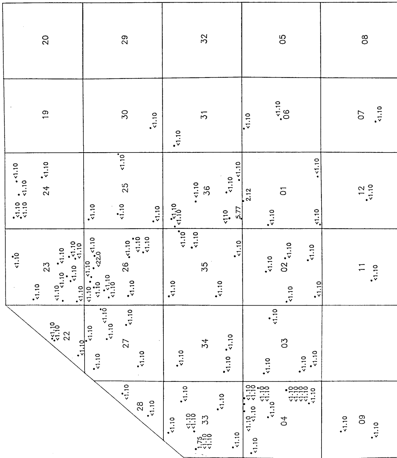
Figure C-99 11DCE CONCENTRATIONS (ug/l) TASK 4, 4th QUARTER ALLUVIAL AQUIFER SOURCE: ESE, 1987
