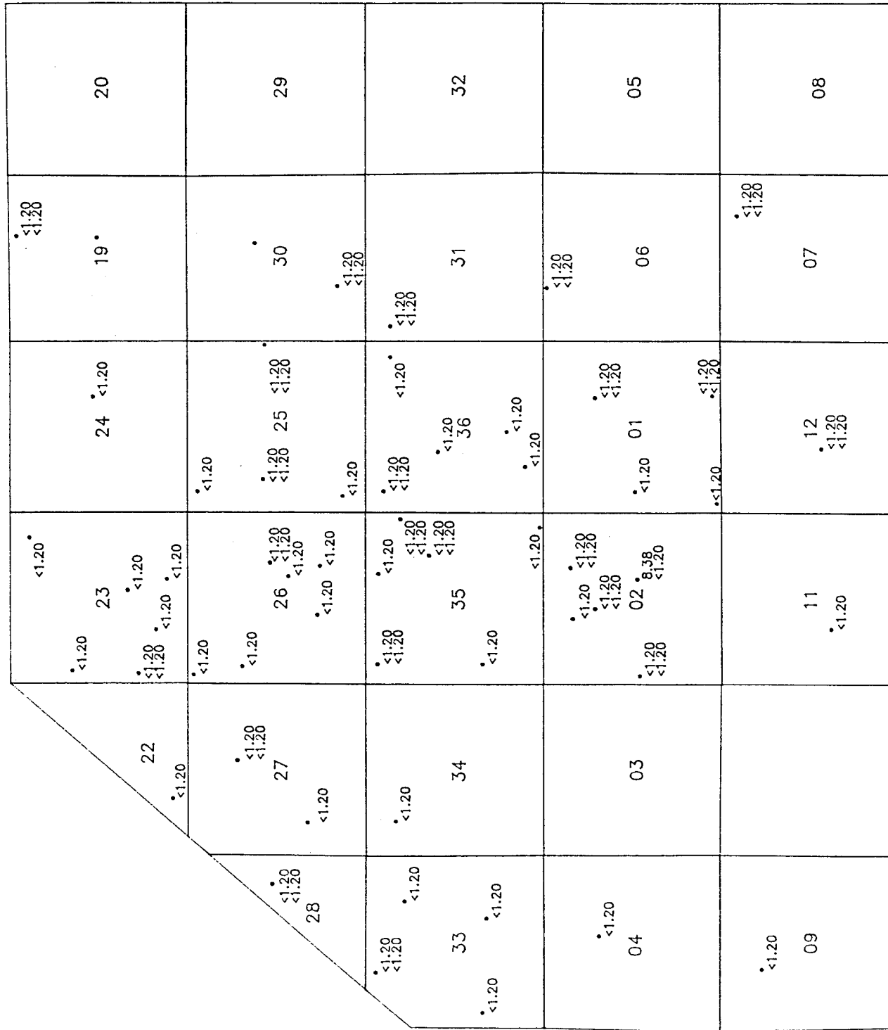
Figure C-102 11DCLE CONCENTRATIONS (ug/l) TASK 4, 3rd QUARTER DENVER AQUIFER SOURCE: ESE, 1987
