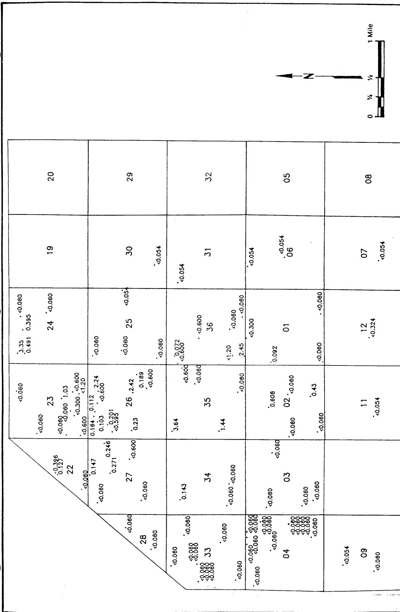
Figure C-19 DIELDRIN CONCENTRATIONS (ug/l) TASK 4 4th QUARTER ALLUVIAL AQUIFER SOURCE: ESE, 1987
