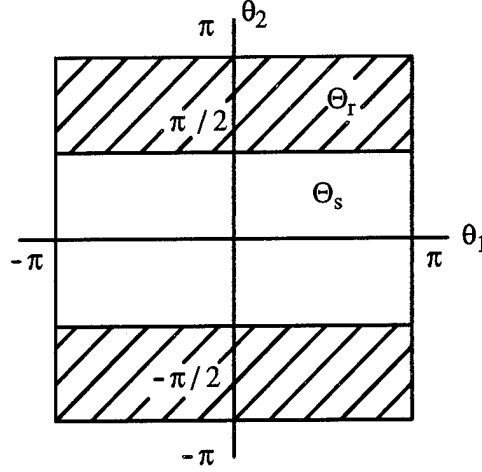
Figure 4.4.2: Smooth ( \Theta_s ) and rough ( \Theta_r , hatched) wavenumber sets in two dimensions, semi-coarsening in x_2 direction.
