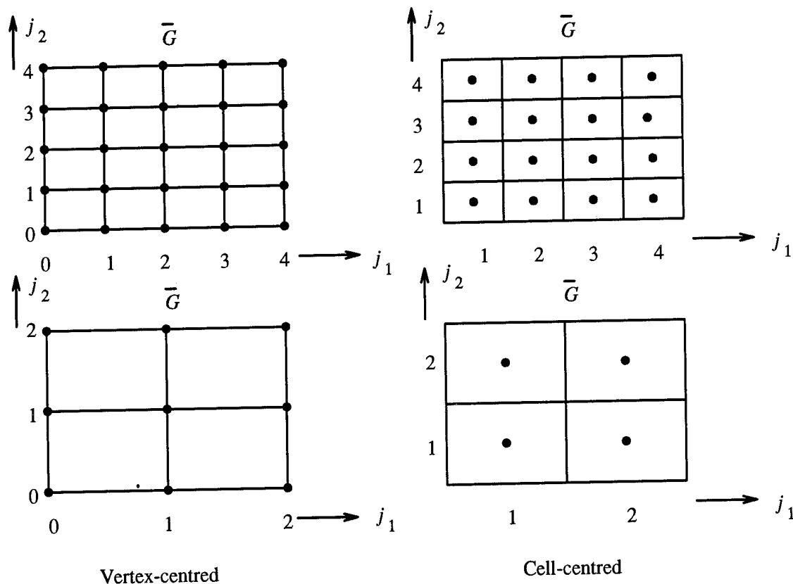
Figure 5.1.2: Vertex-centered and cell-centered coarsening in two dimensions. (• grid points.)
