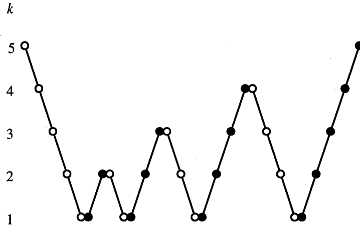
Figure 6.3.3: F-cycle (○ pre-work, ● post-work).
