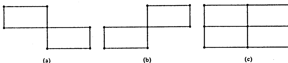
Figure 3.3.3: Discretization stencils.
