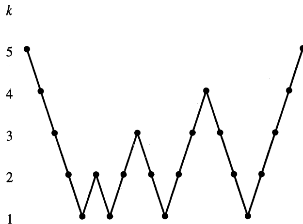
Figure 6.3.2: F-cycle diagram.
