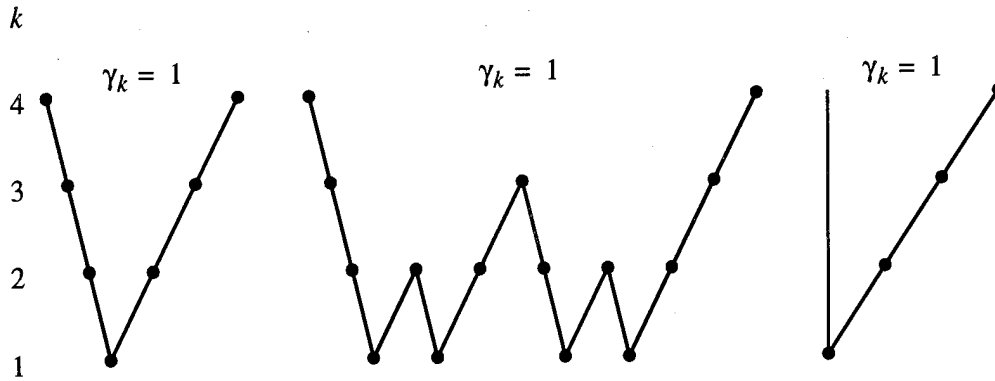
Figure 6.3.1: V-, W- and sawtooth-cycle diagrams.
