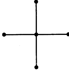
Figure 3.3.4: Five-point stencil.
