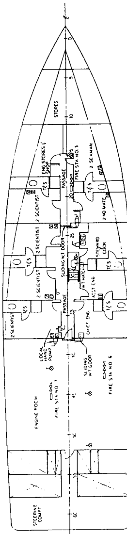
LOWER DECK
