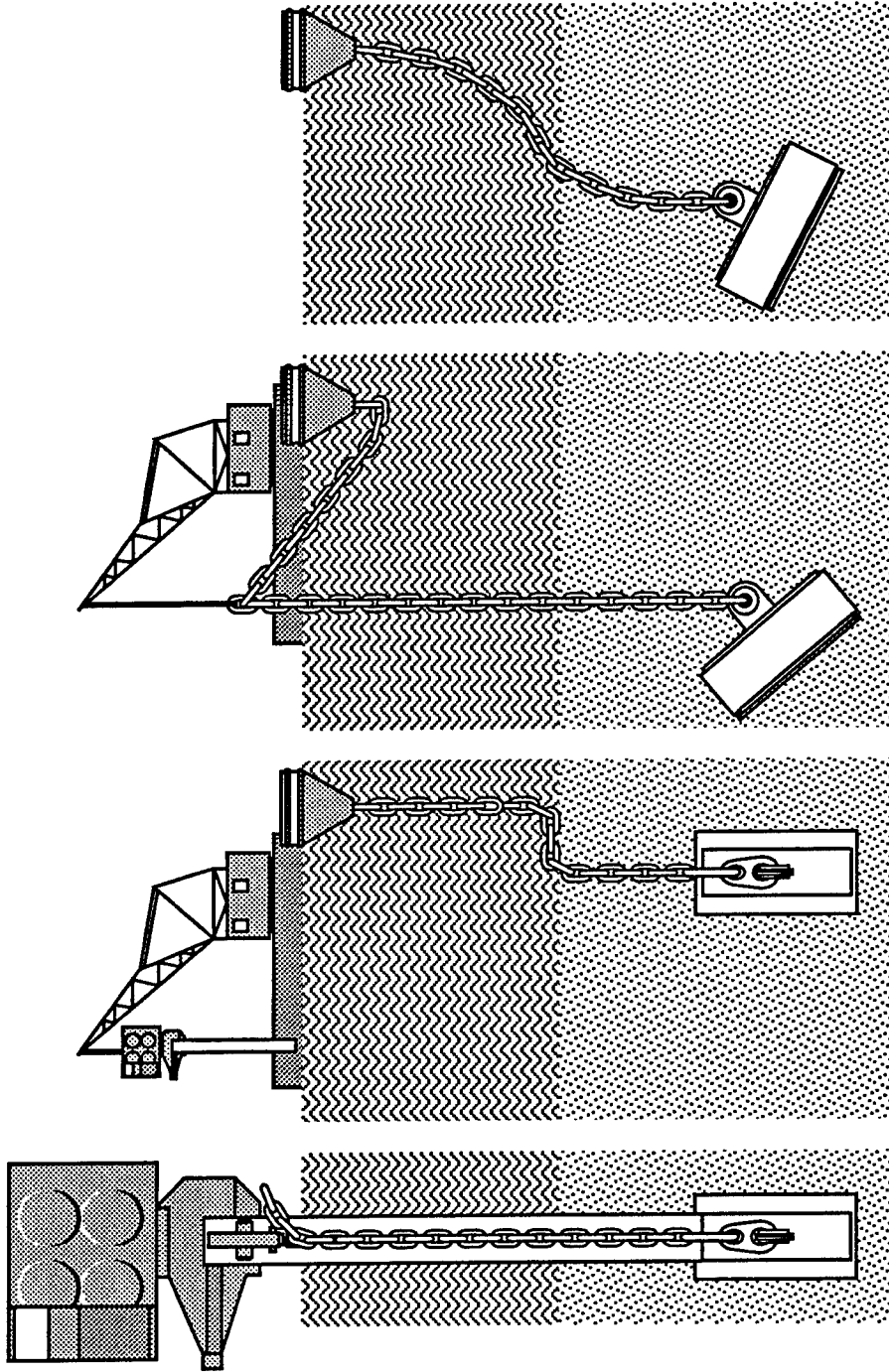
d) Anchor established
