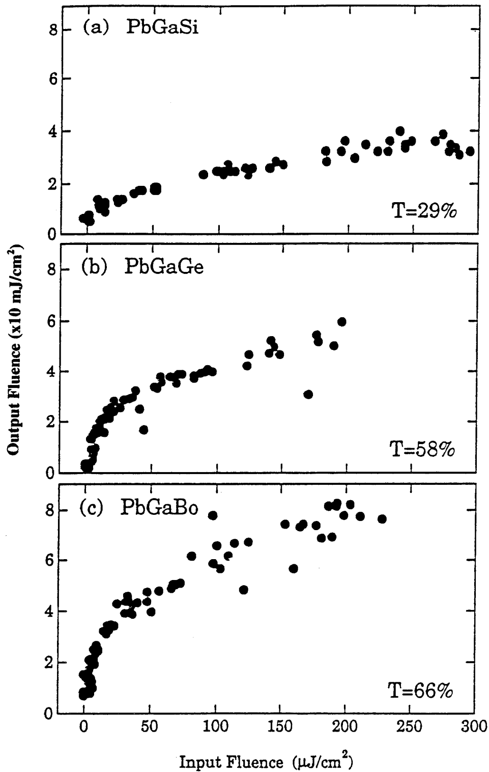
Fig. 2.6. Optical limiting results for samples containing various network formers in the lead gallate ternary system.
