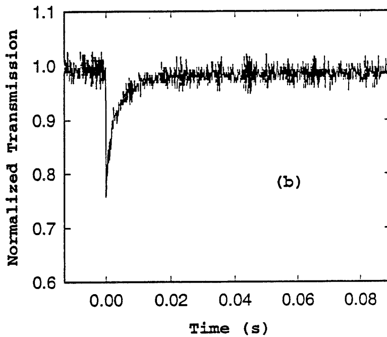
Fig. 4.7. Probe beam depletion following (a) 46.1 \mu\text{J} picosecond excitation and (b) 1.1 \mu\text{J} subpicosecond excitation.
