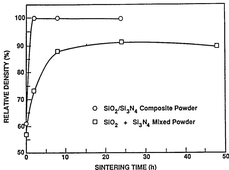
FIG. 3. Plots of relative density vs. sintering time at 1300°C for two types of ~60 vol% \text{SiO}_2 /~40 vol% \text{Si}_3\text{N}_4 powder compacts. Compacts were prepared from (i) a mixture of \text{SiO}_2 particles and \text{Si}_3\text{N}_4 particles and (ii) amorphous silica-coated \text{Si}_3\text{N}_4 particles.
