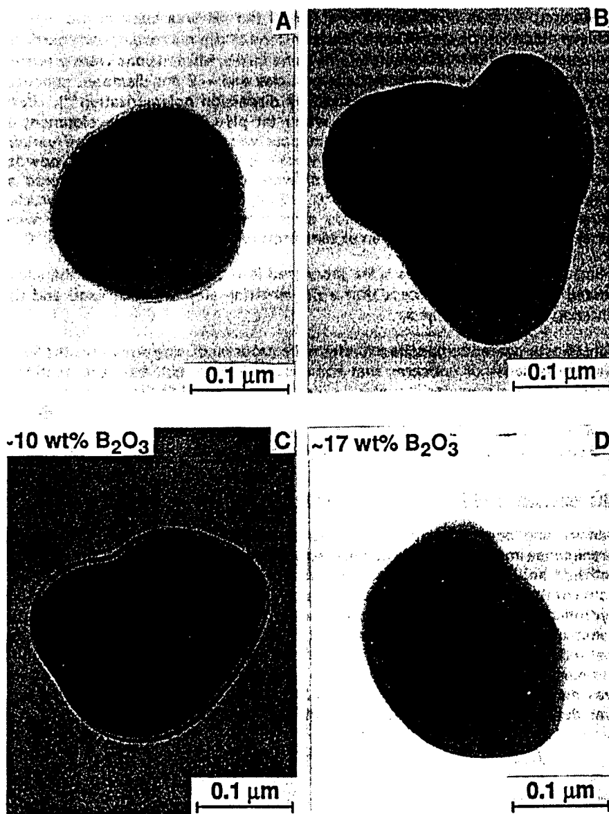
FIG. 2. TEM micrographs of microcomposite particles: (A) SiO 2 /Si 3 N 4 , (B) SiO 2 /Al 2 O 3 , (C) borosilicate (~ 10 wt% B 2 O 3 )/Al 2 O 3 , and (D) borosilicate (~ 17 wt% B 2 O 3 )/Al 2 O 3 .
