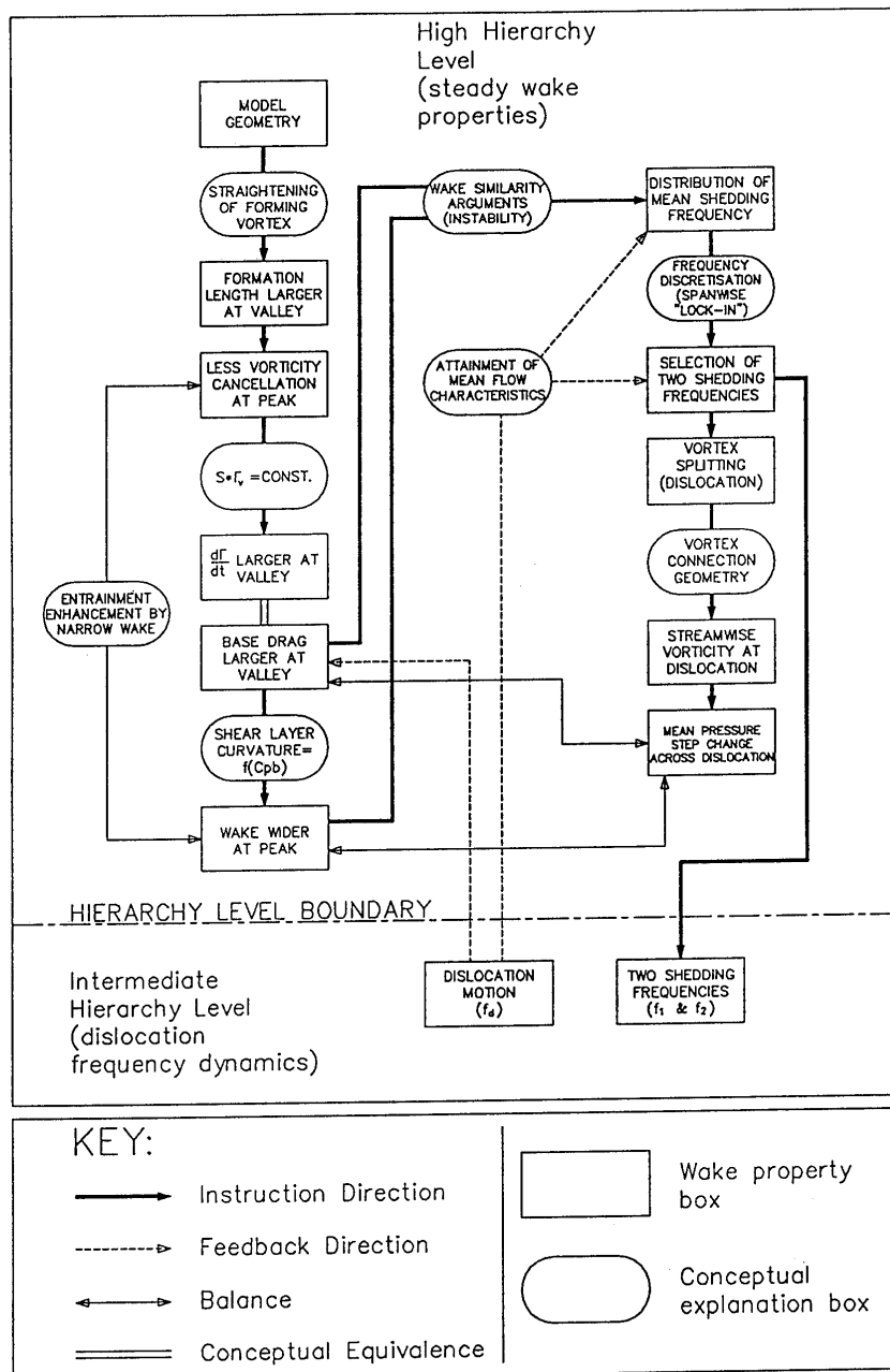
Figure 9.1 Block diagram showing the interaction of wake parameters at the high hierarchy level (steady wake properties).
