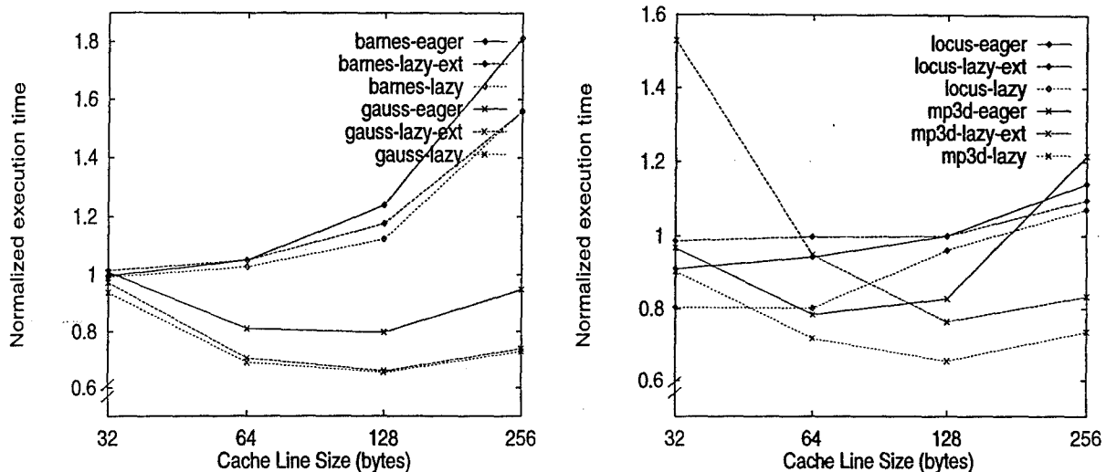
Figure 10: Normalized execution time for different cache line sizes
