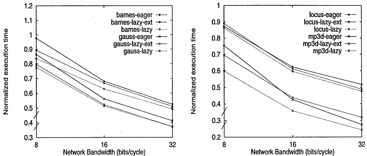
Figure 9: Normalized execution time under different system bandwidths
