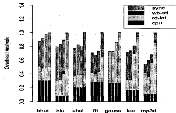
Figure 12: Performance trends for lazy, lazier, and eager release consistency (overhead analysis)
