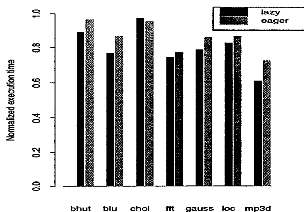
Figure 4: Normalized execution time for lazy-release and eager-release consistency on 64 processors
