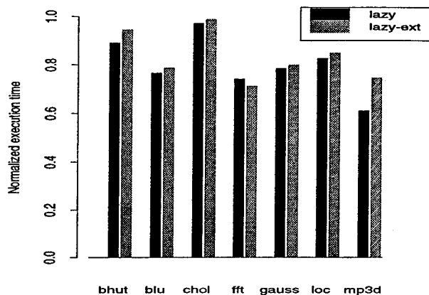
Figure 6: Normalized execution time for lazy-release and lazy-extended-release consistency on 64 processors
