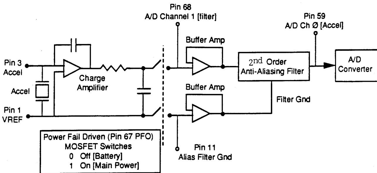
Figure 2-4. Vibration Sensor Circuitry
