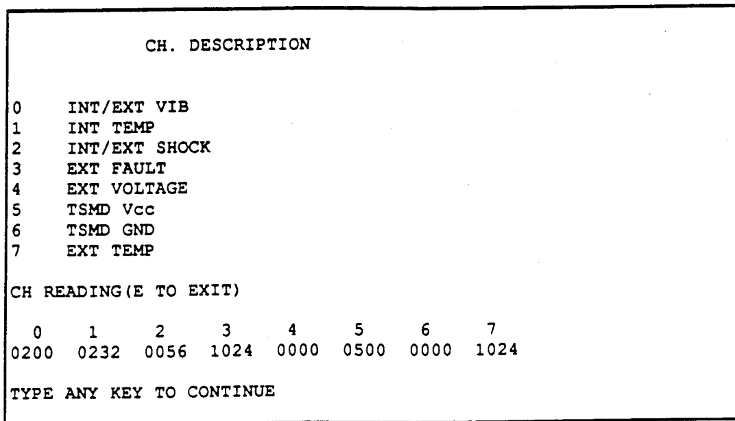
Figure 5-44. A/D Display
