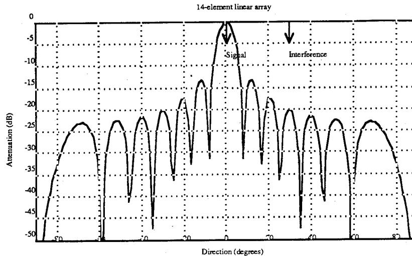
FIGURE 1 Beam pattern for a uniformly weighted linear array
