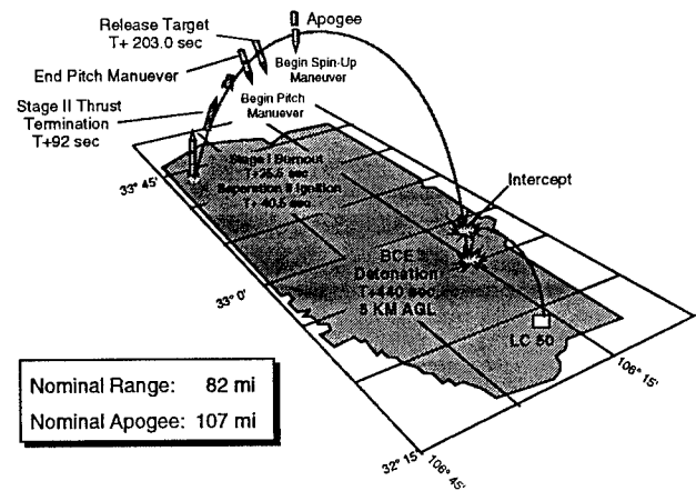
Figure 14: STORM BTTV Mission Overview at WSMR
