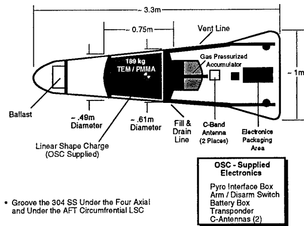
Figure 11: STORM BTTV Bulk Chemical Experiment Reentry Vehicle
