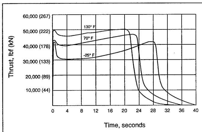
Figure 5: Sergeant XM100 Thrust vs. Time
