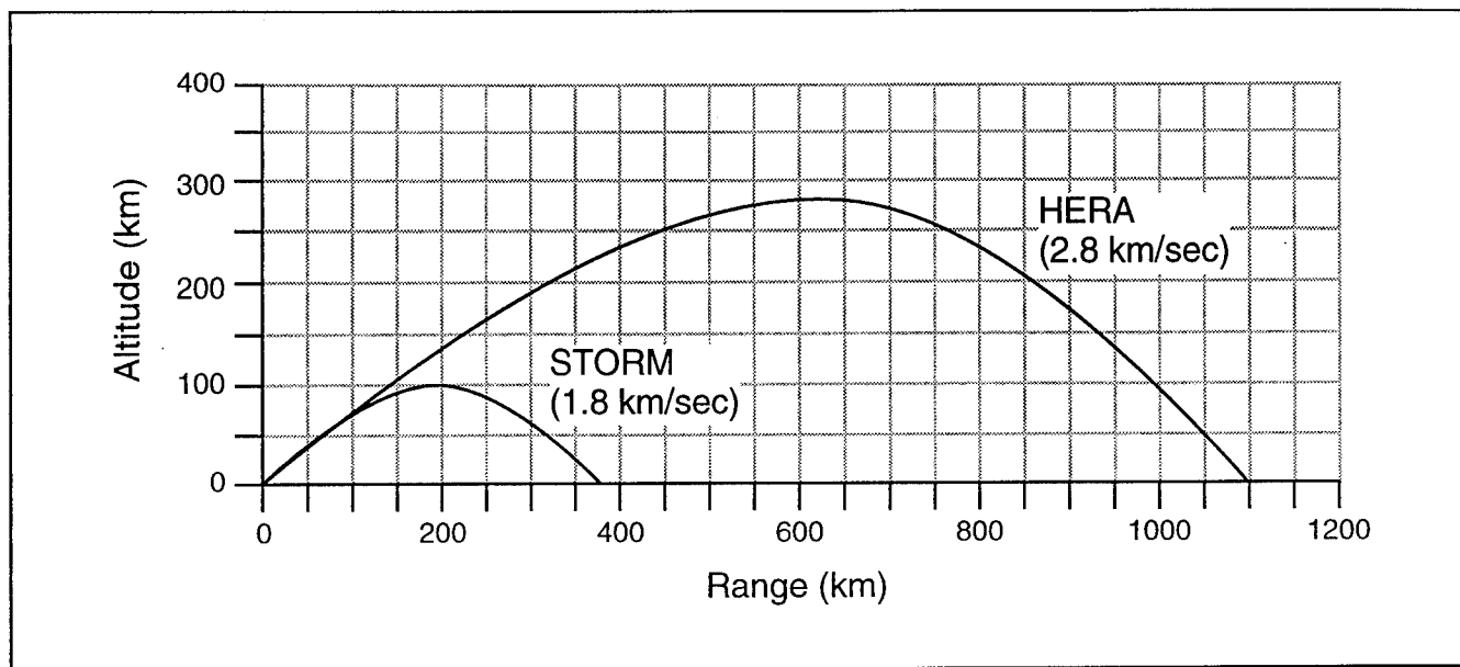
Figure #1: Theater Target Trajectories
