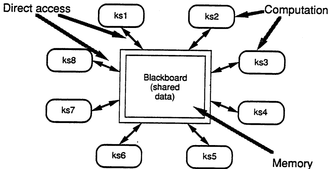
Figure 4: The Blackboard
