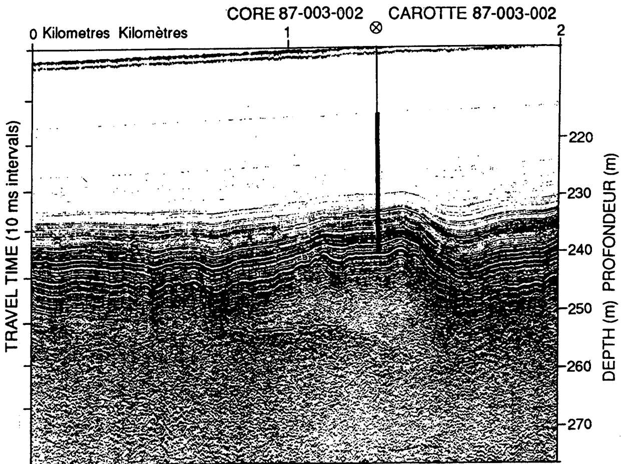
Figure 19: Huntex deep tow seismic reflection profile at DREA experimental site 2 in Emerald Basin [Moran et al., 1991]. Core 87-003-002 location is superimposed (physical properties are in Fig. 24).
