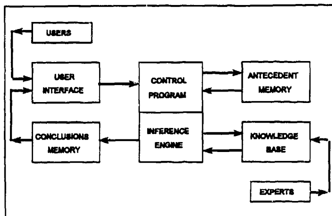
Figure 16. Components of a knowledge-based expert system
