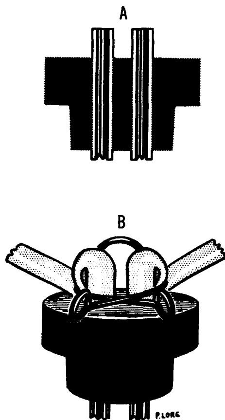
FIGURE 36.—Application of clamp to Red Cross donor bottle when collection of blood is complete. A. Airway and bleeding tube. B. Bottle tubes clamped off.
