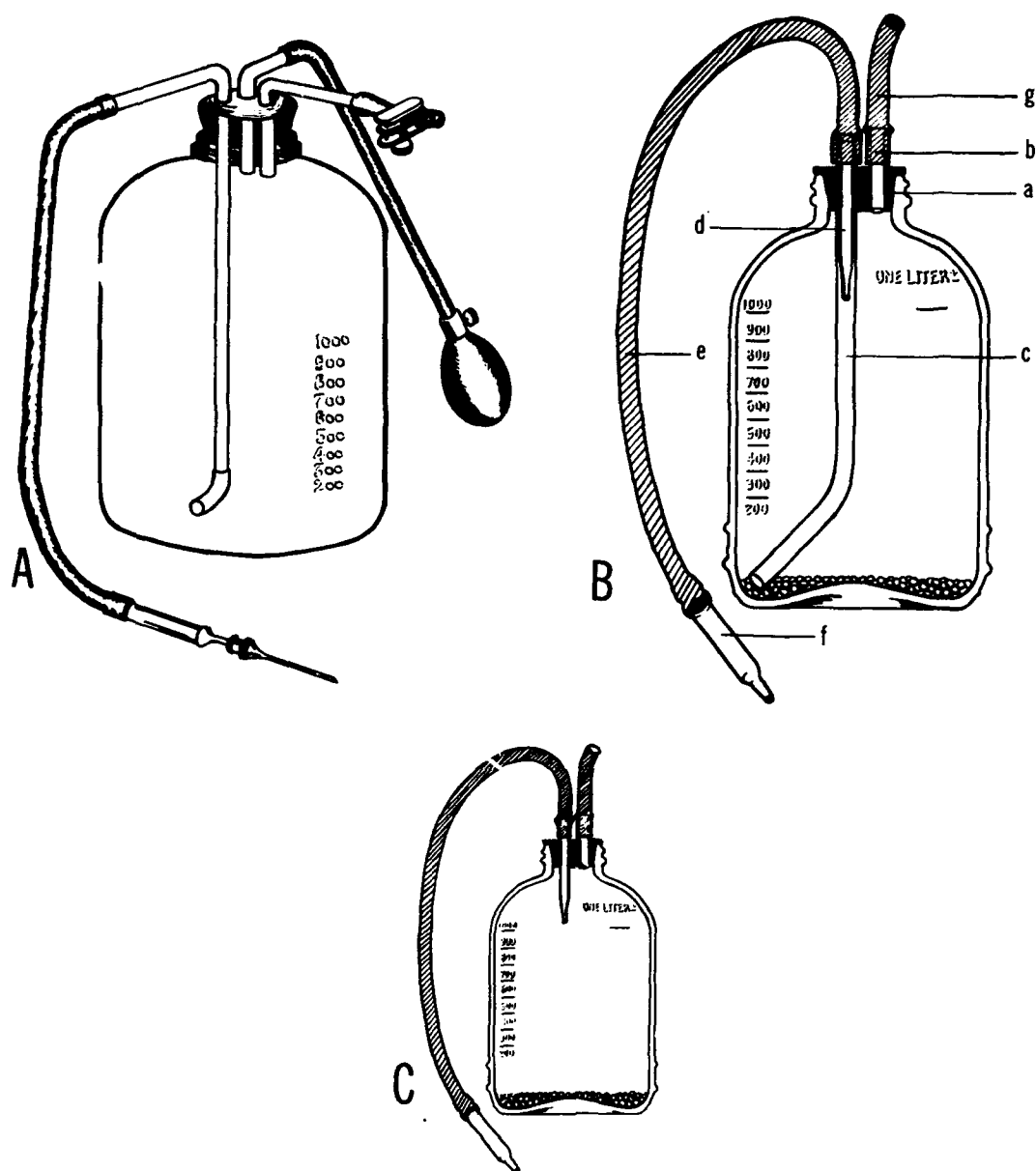
FIGURE 47.—Evolution of donor bottle in Ebert-Emerson transfusion set. A. First model. B. Second model: Rubber stopper with two holes (a); medicine dropper, cut to 1\frac{1}{8} inches (b); glass tube, 10-mm. diameter, 8\frac{1}{4} inches long (c); medicine dropper (d); gum rubber tube, 14 inches long (e); adapter for Luer needle (f); gum rubber tube, 3 inches long (g). C. Final model, with long glass tube eliminated.
