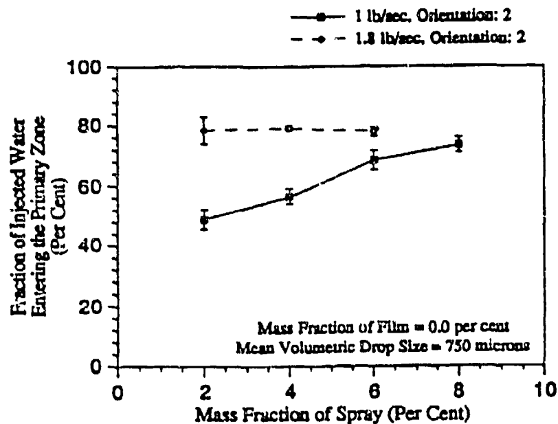
Figure 33. Case IV: Effect of Mass Fraction of Injected Spray of Large Droplet Size on Water Entry into the Primary Zone Through the Dome and Primary Jets (Orientation 2)
