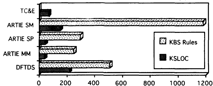
Figure 3-10 Representative AI Applications Written in Ada
