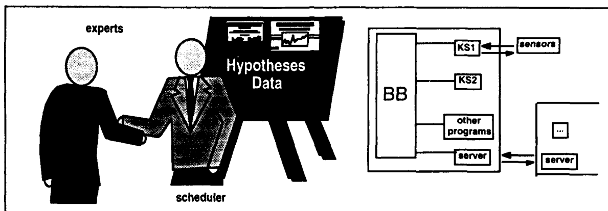
Figure 3-6 The Blackboard Architecture
