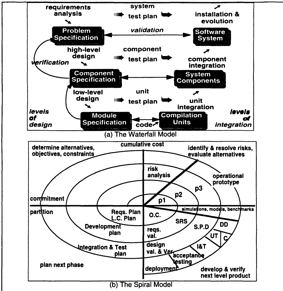
Figure 3-1 Conventional Software Development Process Models
