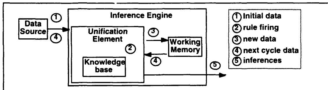
Figure 3-5 A Simple Inference Engine
