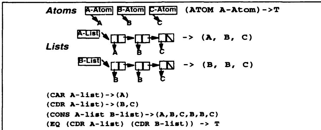
Figure 3-4 Pure LISP Basic Elements
