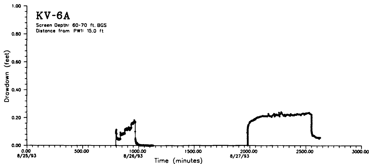
Figure 4-3. Pumping Test Hydrograph for Wells PW-1, KV-2 and KV-6A
