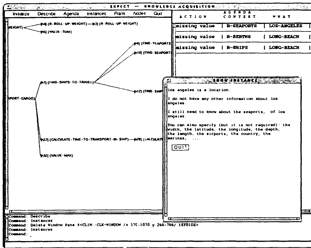
Figure 3: EXPECT's user interface.
