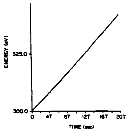
FIG. 20. Total energy versus time for \delta = 0.01 , \nu_c T = 0.2 , E_0 = 300 eV, and a sawtooth perturbation.
