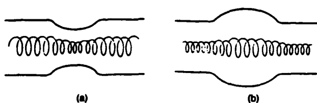
FIG. 2. Particle orbits in a sinusoidally perturbed magnetic field. (a) Plasma compressed during the positive half-cycle, (b) plasma relaxed during the negative half-cycle.
