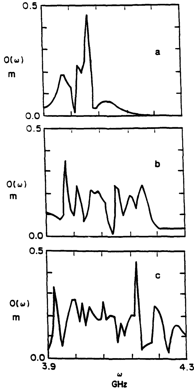
Fig. 5. Back-scattering cross-section versus wave frequency, \theta = 60^\circ , \Omega = 4 GHz, v = 20 MHz: (a) N_0 = 1015 \text{ m}^{-3} , (b) N_0 = 51015 \text{ m}^{-3} , (c) N_0 = 1016 \text{ m}^{-3} .
