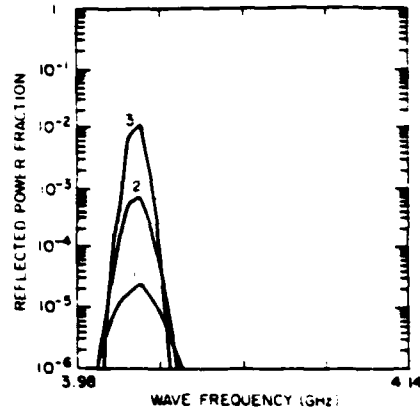
Fig. 7. Reflected power per unit incident power versus wave frequency, \theta = 60^\circ ; \Omega = 4 GHz; N_o = 10^{15} \text{ m}^{-3} : (1) \nu = 20 MHz, (2) \nu = 10 MHz, (3) \nu = 5 MHz.
