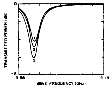
Fig. 15. Transmitted power versus wave frequency, \Omega = 4 GHz; N_o = 10^{15} \text{ m}^{-3} ; \nu = 10 MHz: (1) \theta = 90^\circ , (2) \theta = 72^\circ , (3) \theta = 60^\circ .
