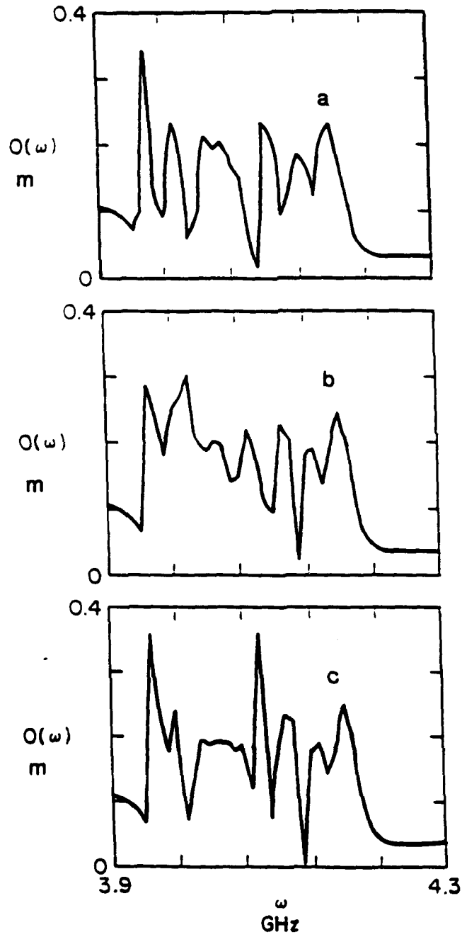
Fig. 4. Back-scattering cross-section versus wave frequency, \theta = 60^\circ , \Omega = 4 GHz, N_0 = 51015 \text{ m}^{-3} : (a) \nu = 5 MHz, (b) \nu = 20 MHz, (c) \nu = 10 MHz.
