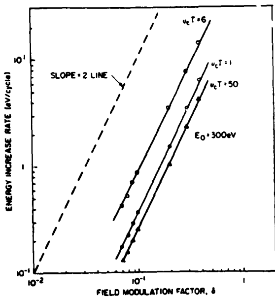
FIG. 7. Energy increase rate versus field modulation factor for E_0 = 300 eV, several collisionality parameters, and a sinusoidal perturbation.
