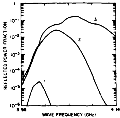
Fig. 8. Reflected power per unit incident power versus wave frequency, \theta = 60^\circ ; \Omega = 4 GHz; \nu = 20 MHz: (1) N_o = 10^{15} \text{ m}^{-3} , (2) N_o = 5 \cdot 10^{15} \text{ m}^{-3} , (3) N_o = 10^{16} \text{ m}^{-3} .
