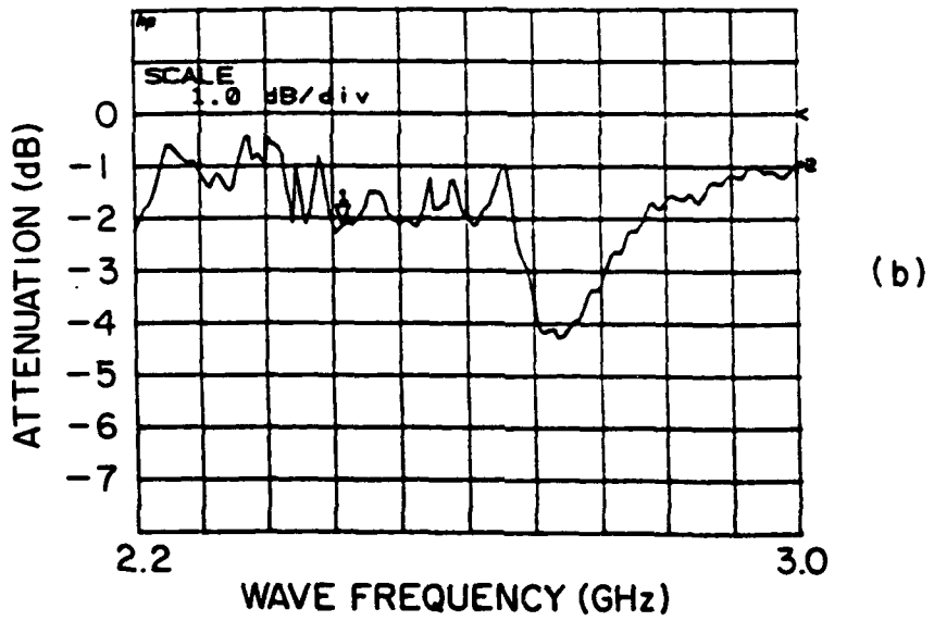
Fig.10 Attenuation Vs. frequency for V=700V ; P=70mTorr ; (a) B=950 Gauss, (b) B=970 Gauss.
