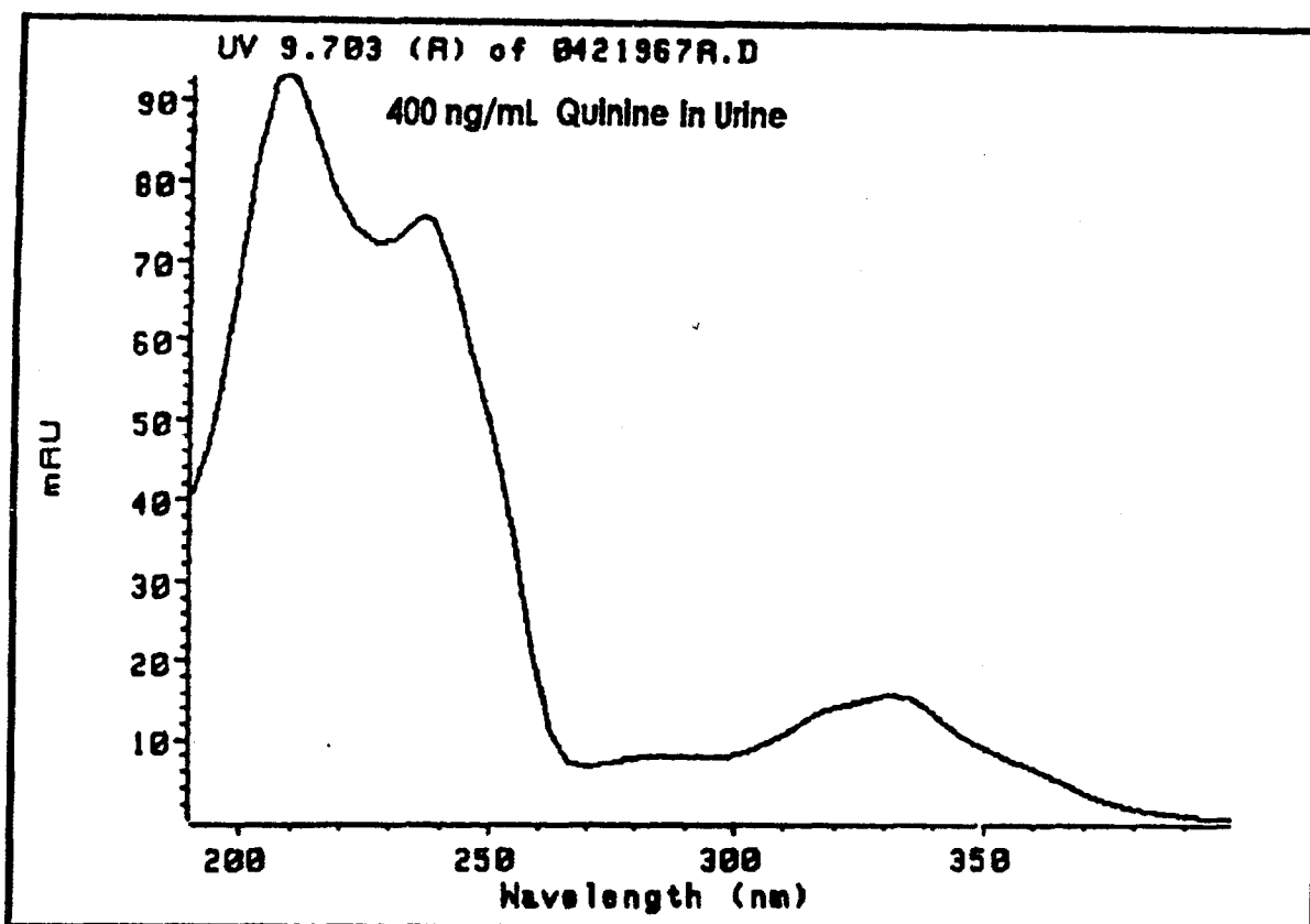
Figure 2. UV spectra of quinine
