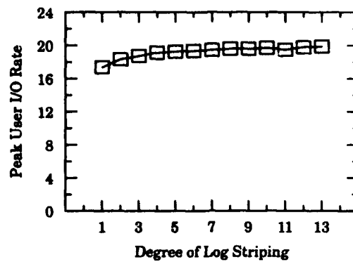
Figure 17(a): Peak user I/Os
