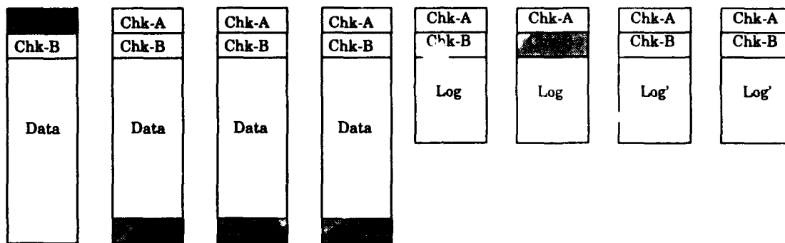
Fig. 25. A parity-logging array that uses a nonbinary code to achieve double-fault tolerance. By using nonbinary codes, disk arrays can achieve double failure tolerance with only two disks of check data. Shown above is a single region of a double fault tolerant parity logging disk array with nonbinary check information. The parity of a single fault tolerant array is replaced with two sets of check information. The shaded area shows an example pair of check information blocks and the data blocks that they protect.
