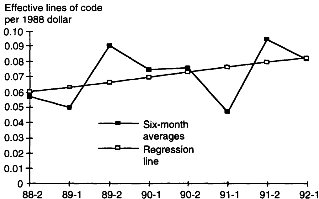
Figure 14. Effective Lines of Code per 1988 Dollar
