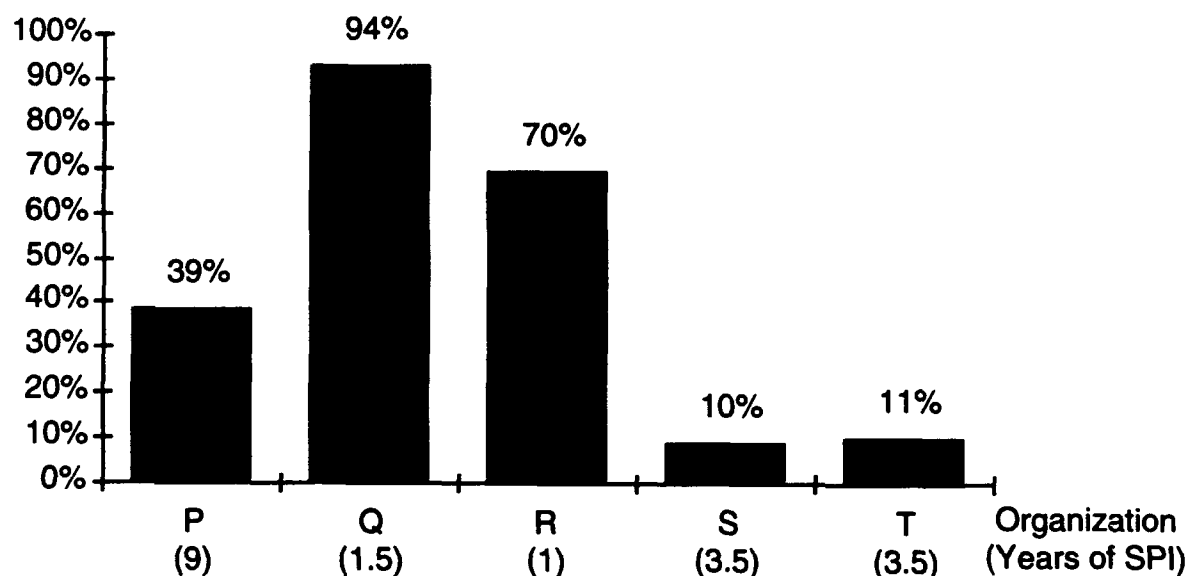
Figure 7. Reduction per Year in Post-release Defect Reports
