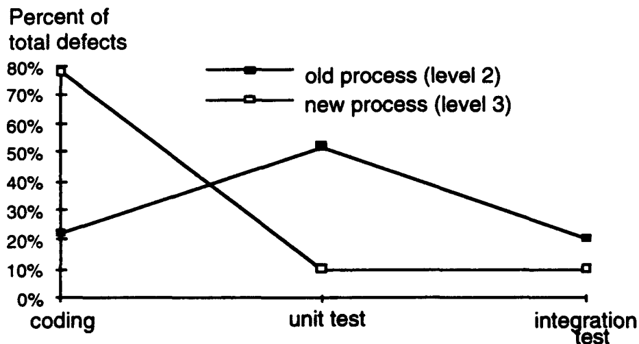
Figure 10. Percentage of Defects Found by Stage
