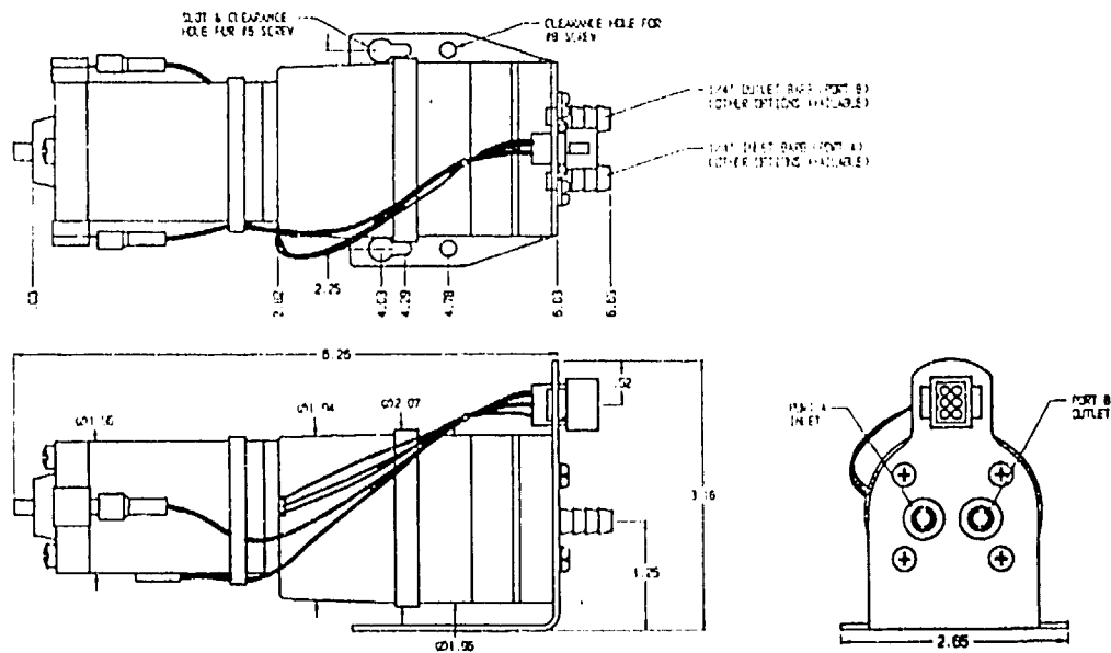
Figure 6.2 Xolox Gear Type Fuel Pump
