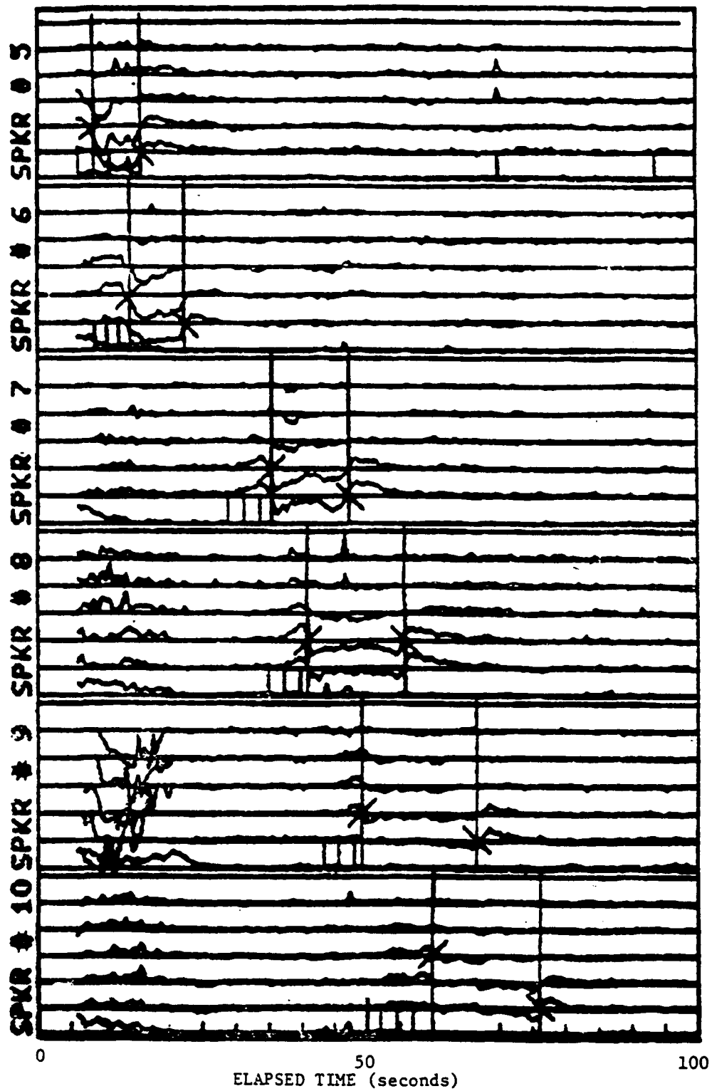
FIGURE 2-6. SAMPLE VORTEX DETECTION CORRELATIONS
