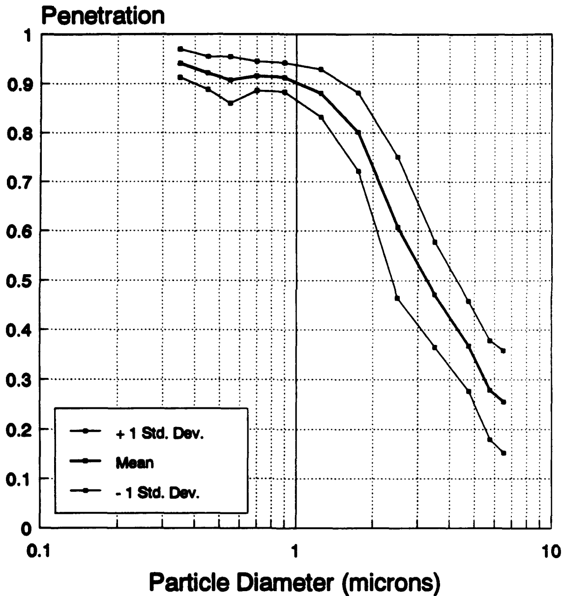
Figure 12. Mean and +/- 1 standard deviation penetration curves for Fabric D.
