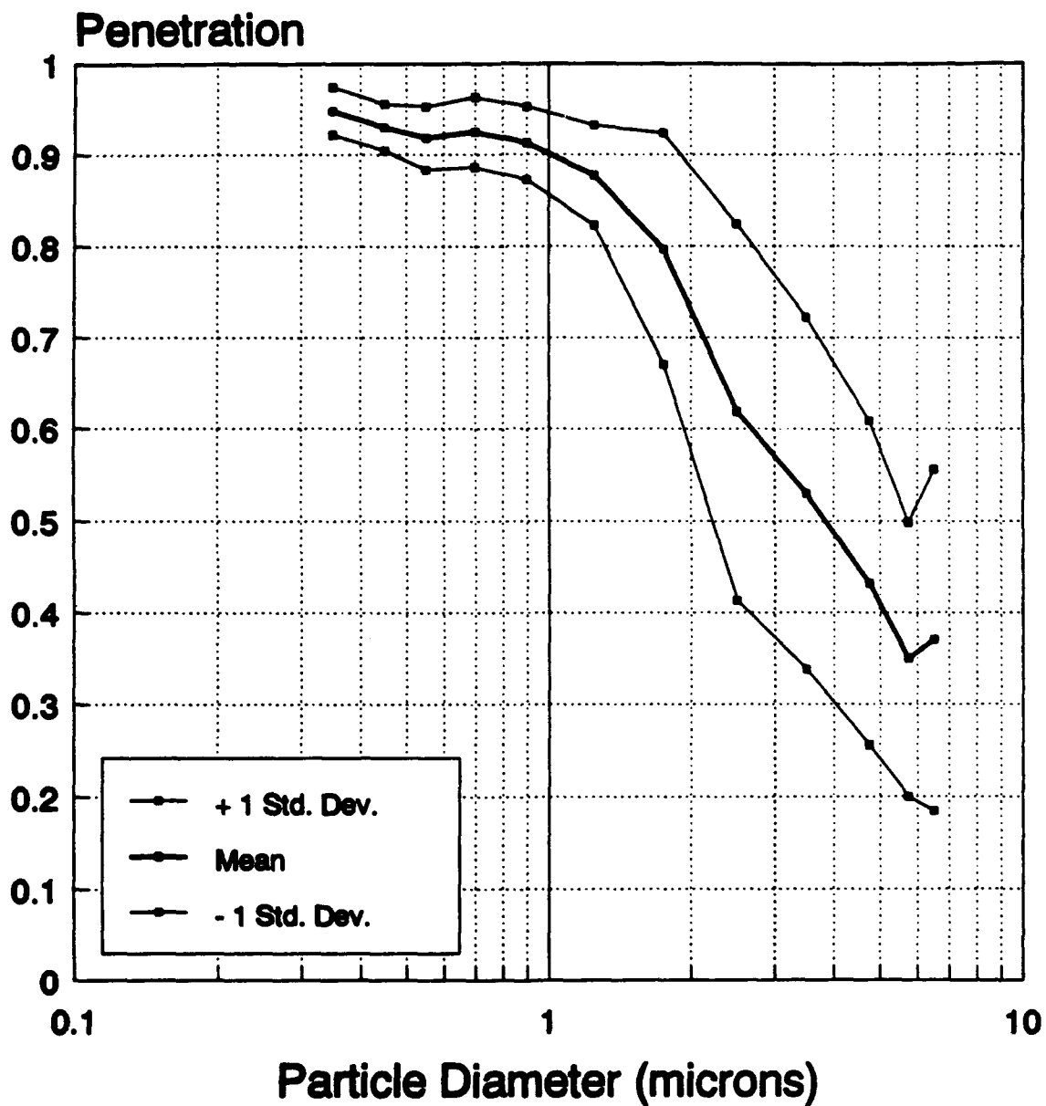
Figure 10. Mean and +/- 1 standard deviation penetration curves for Fabric B.
