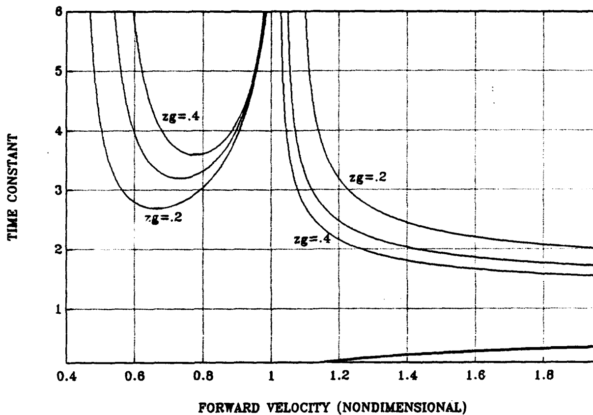
FIGURE 4.10 The effects of changing zq on the bifurcation maps, xq=.1 .
