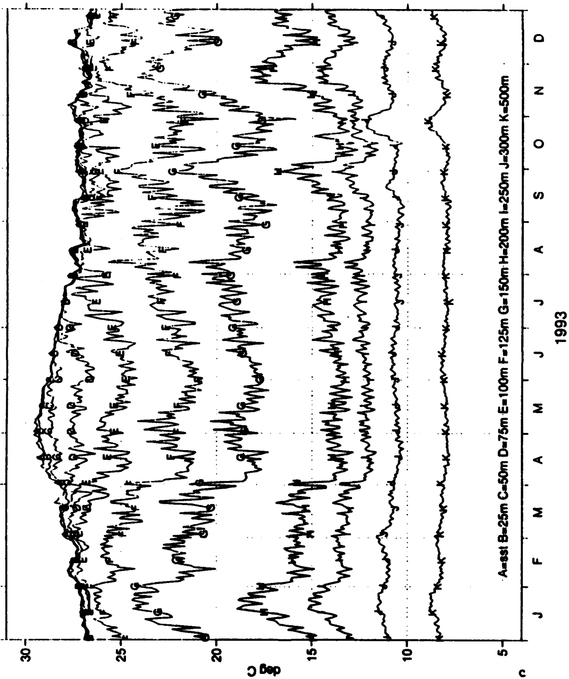
Subsurface Temperature Time Series, 5S140W
