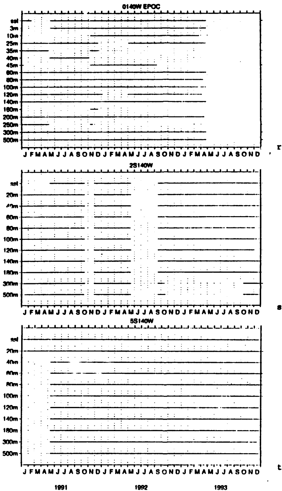
Fig. 11. (Continued) r) 0^{\circ} 140^{\circ} W, s) 2^{\circ} S 140^{\circ} W, t) 5^{\circ} S 140^{\circ} W,
