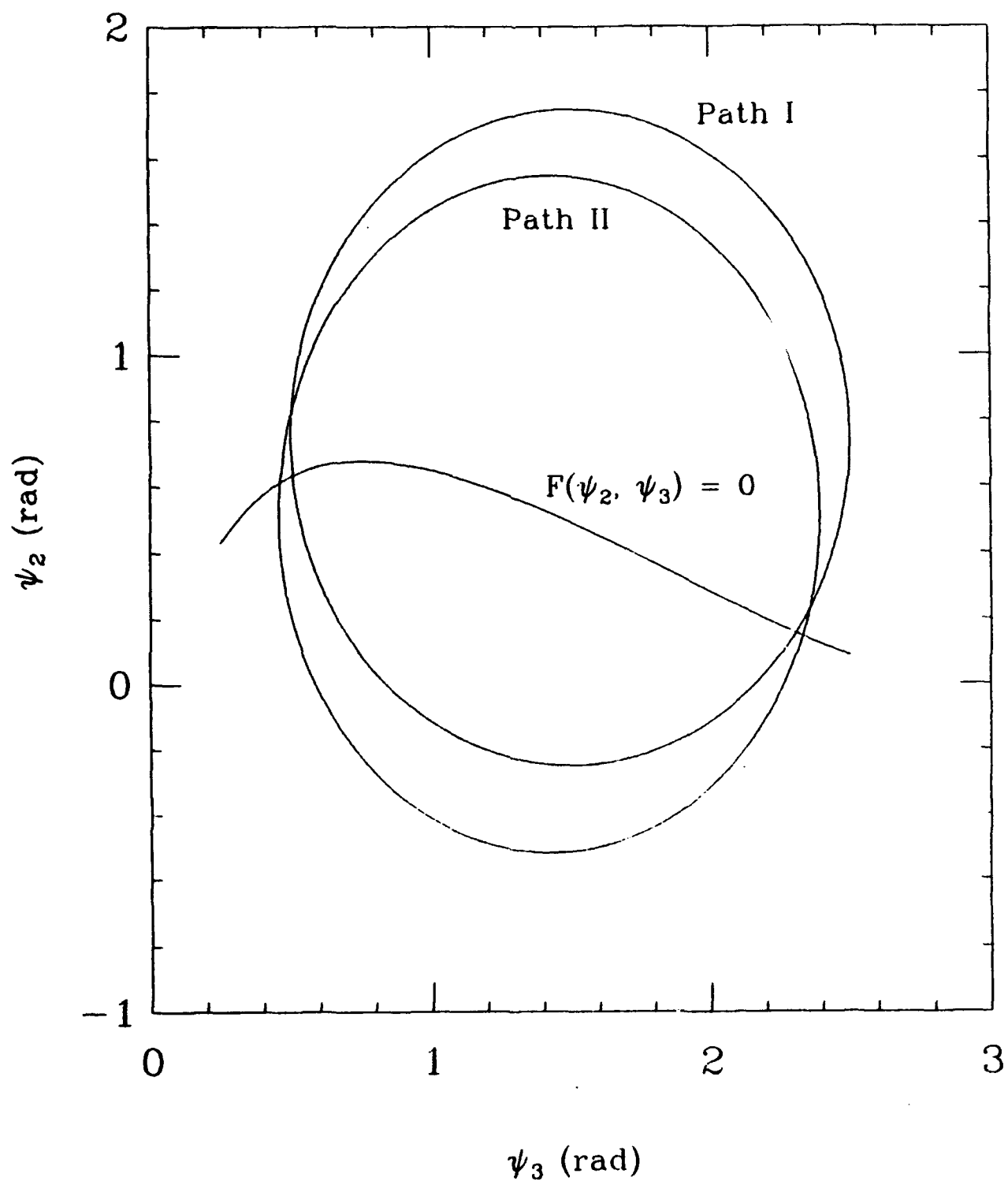
Figure 11. Elliptical paths in the space of the independent joint variables of the three link redundant robot. Path I is the initially chosen path and Path II is the optimized path.
