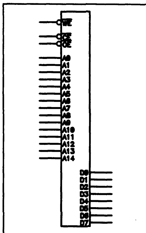
Figure 11 TMS29F258-20NJQ4
