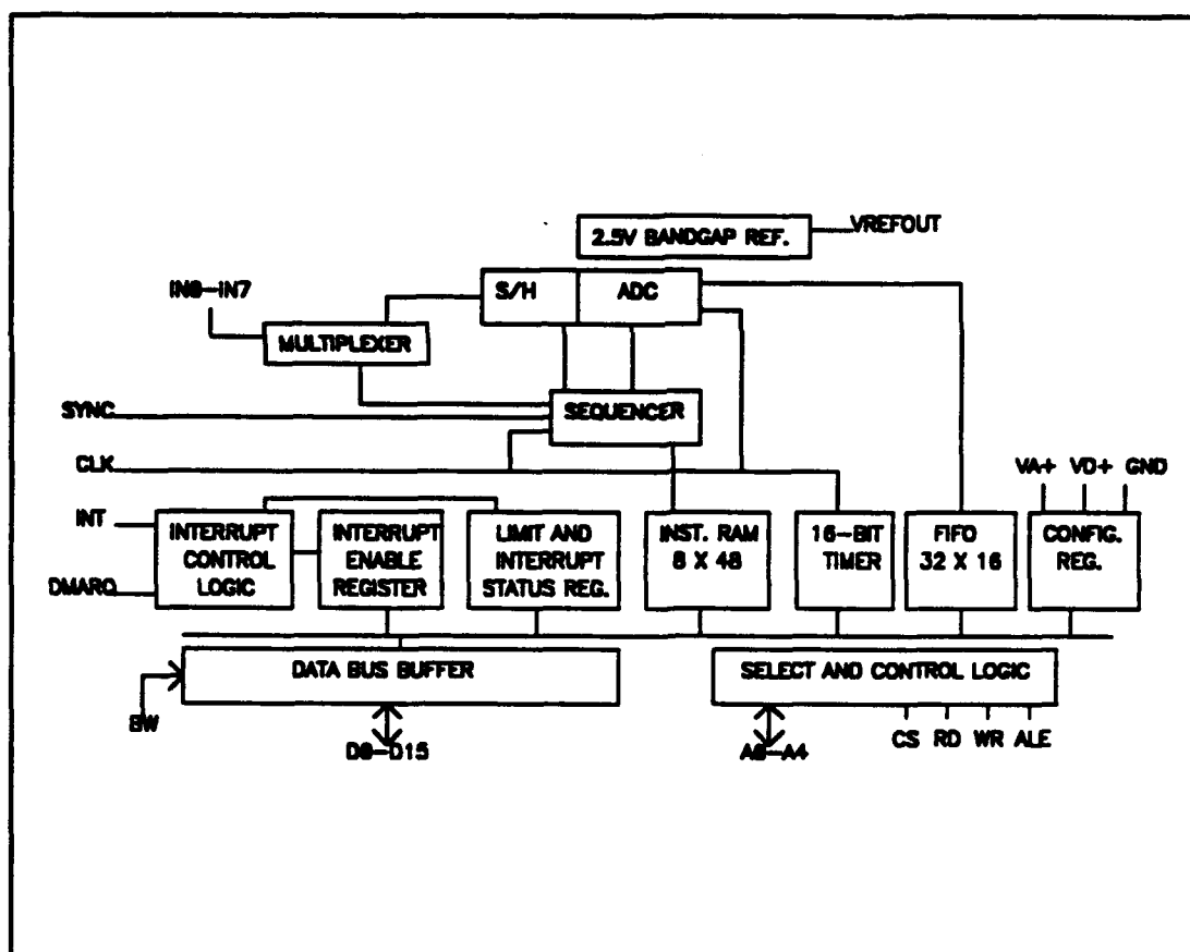
Figure 31 ADC Functional Diagram
