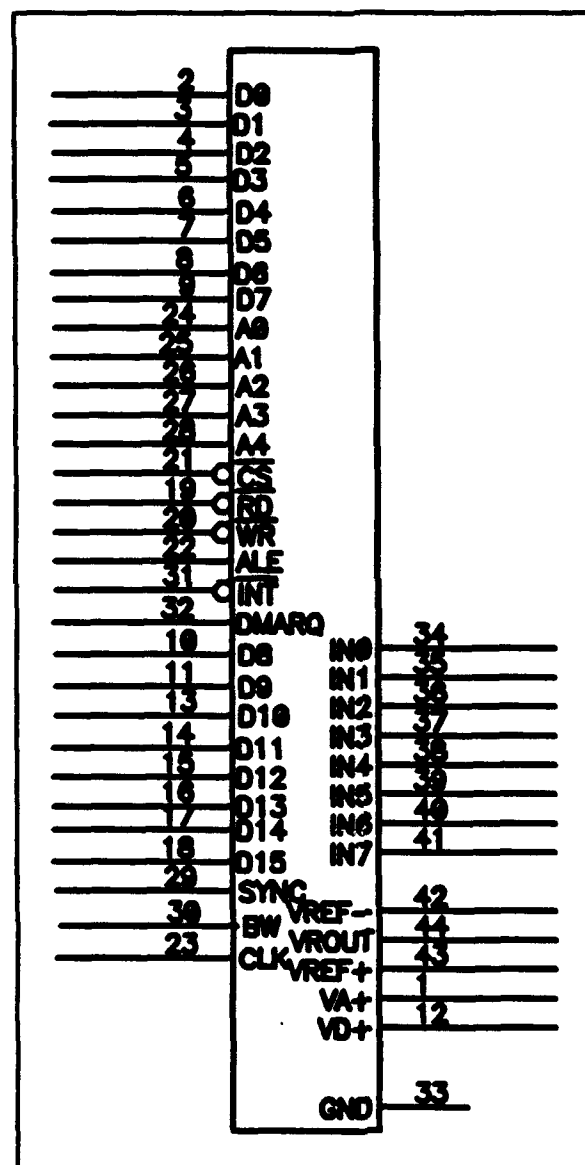
Figure 30 LM12H454
