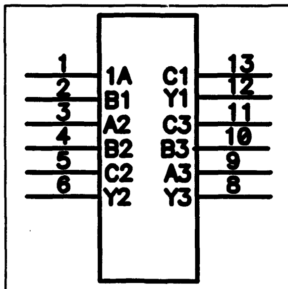
Figure 21 HCS27MS
