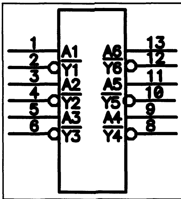
Figure 28 HCS04MS
