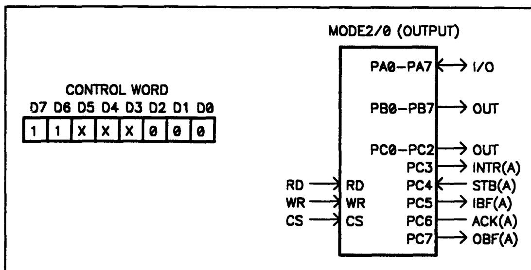
Figure 6 PPI OPERATION
