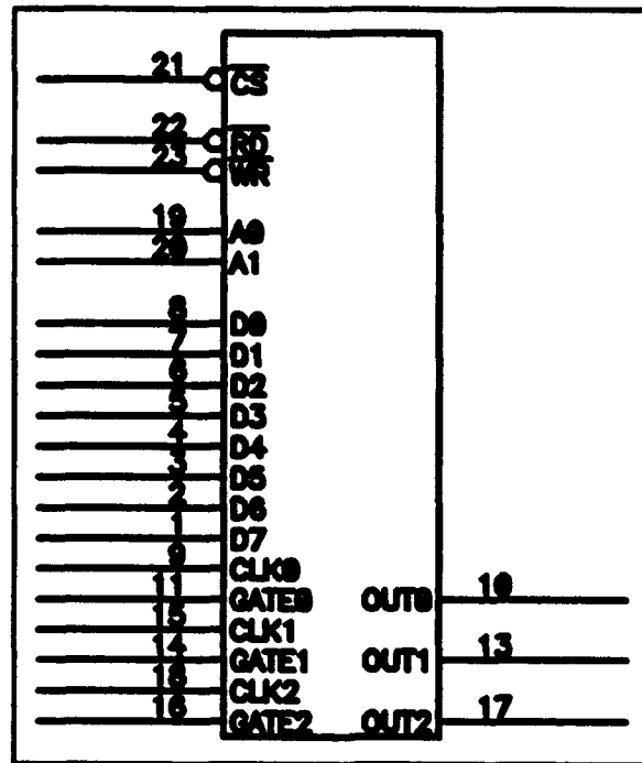
Figure 32 82C54-2
