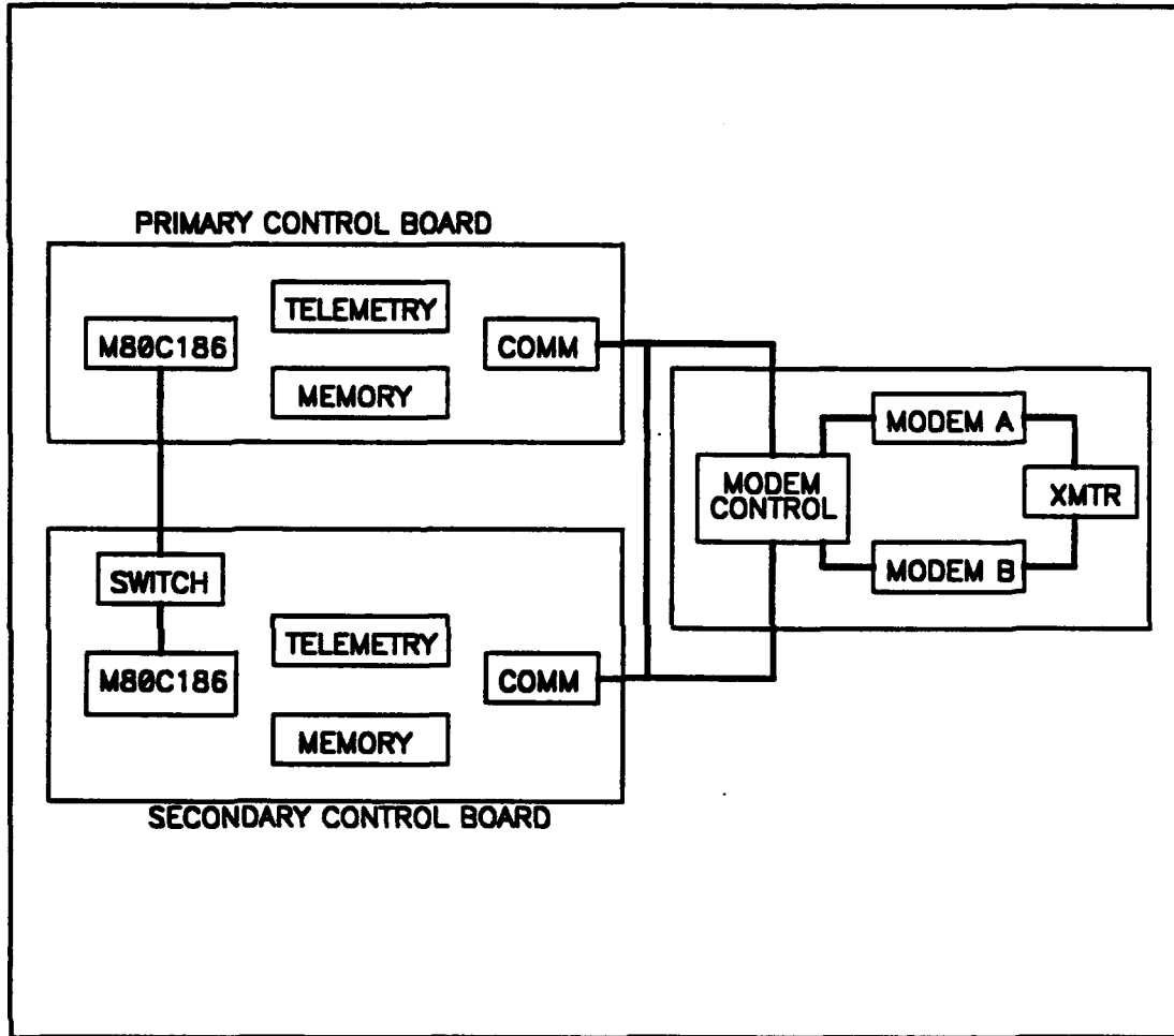
Figure 2 Preliminary DCS Design [Ref. 5: p. 2]
