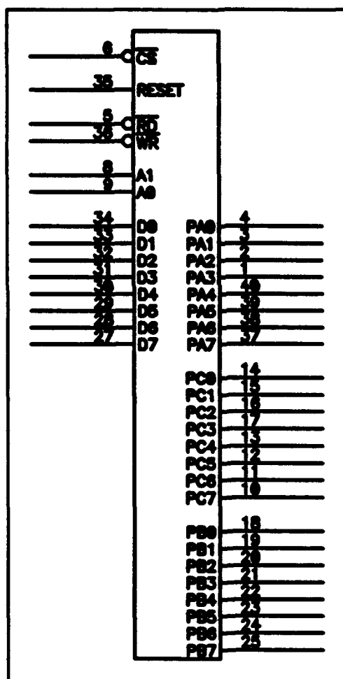
Figure 5 82C55A
