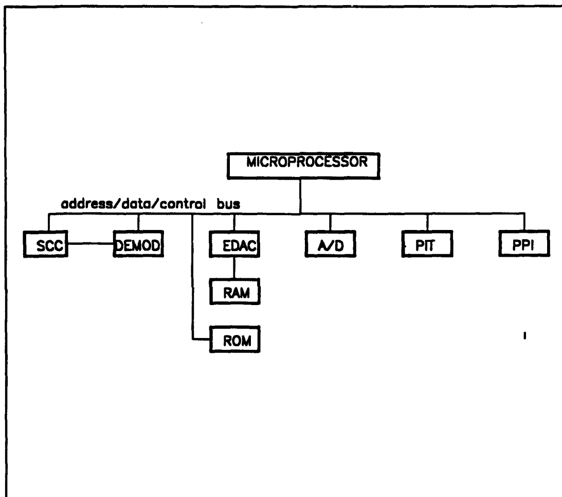
Figure 3 Current DCS Design
