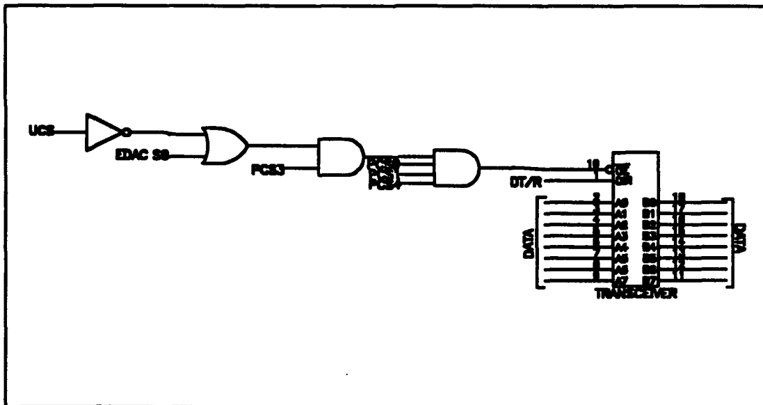
Figure 26 Transceiver Connectivity
