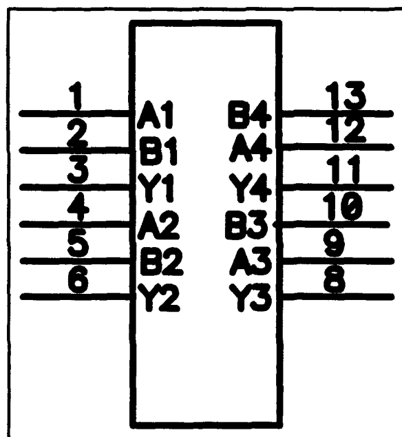
Figure 22 HCS00MS
