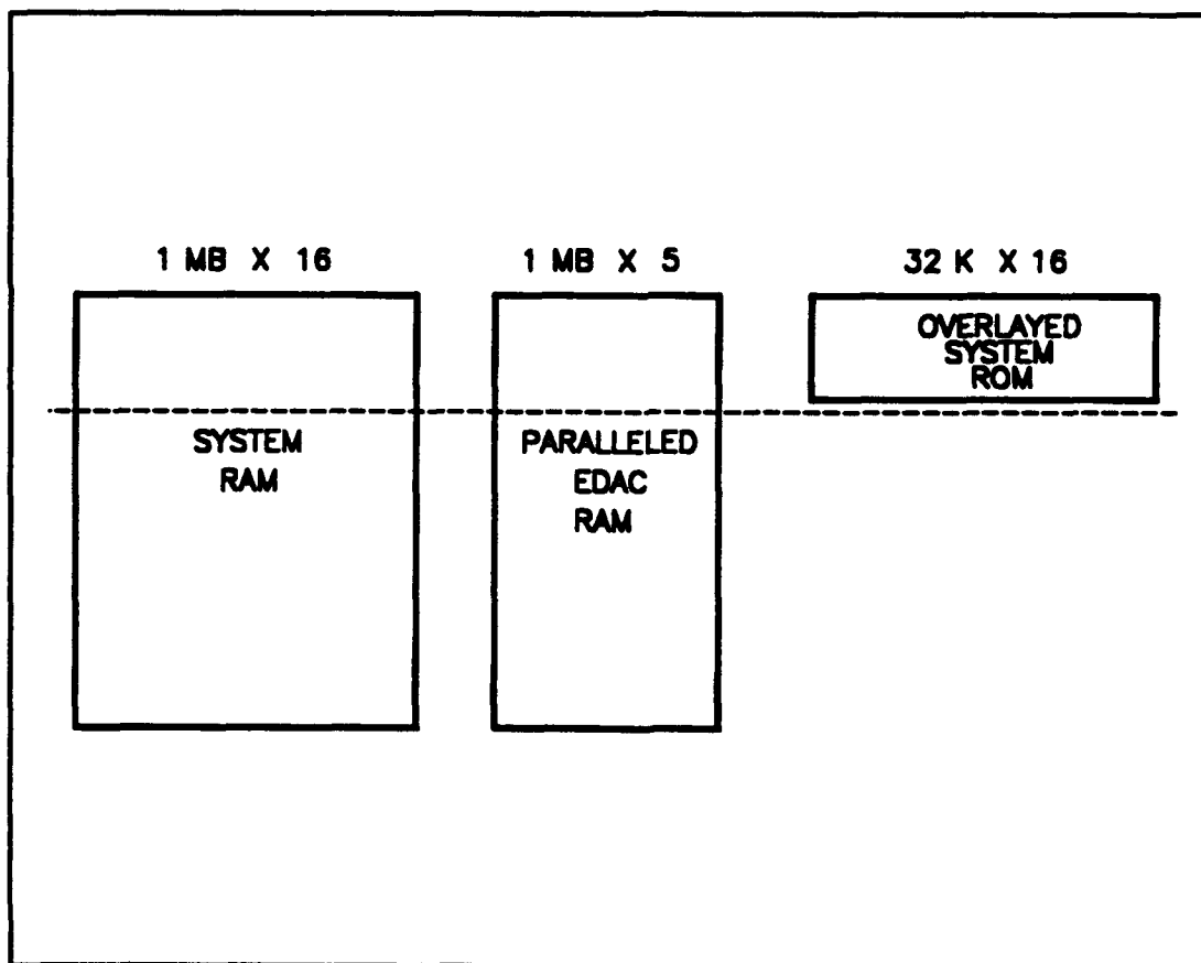
Figure 10 System Memory Map
