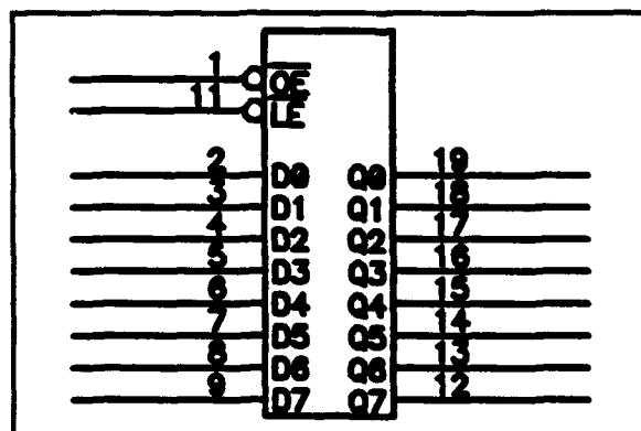
Figure 29 HCS573MS
