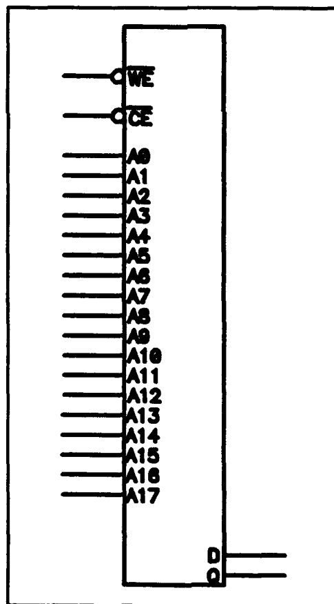
Figure 17 EDI81256C
