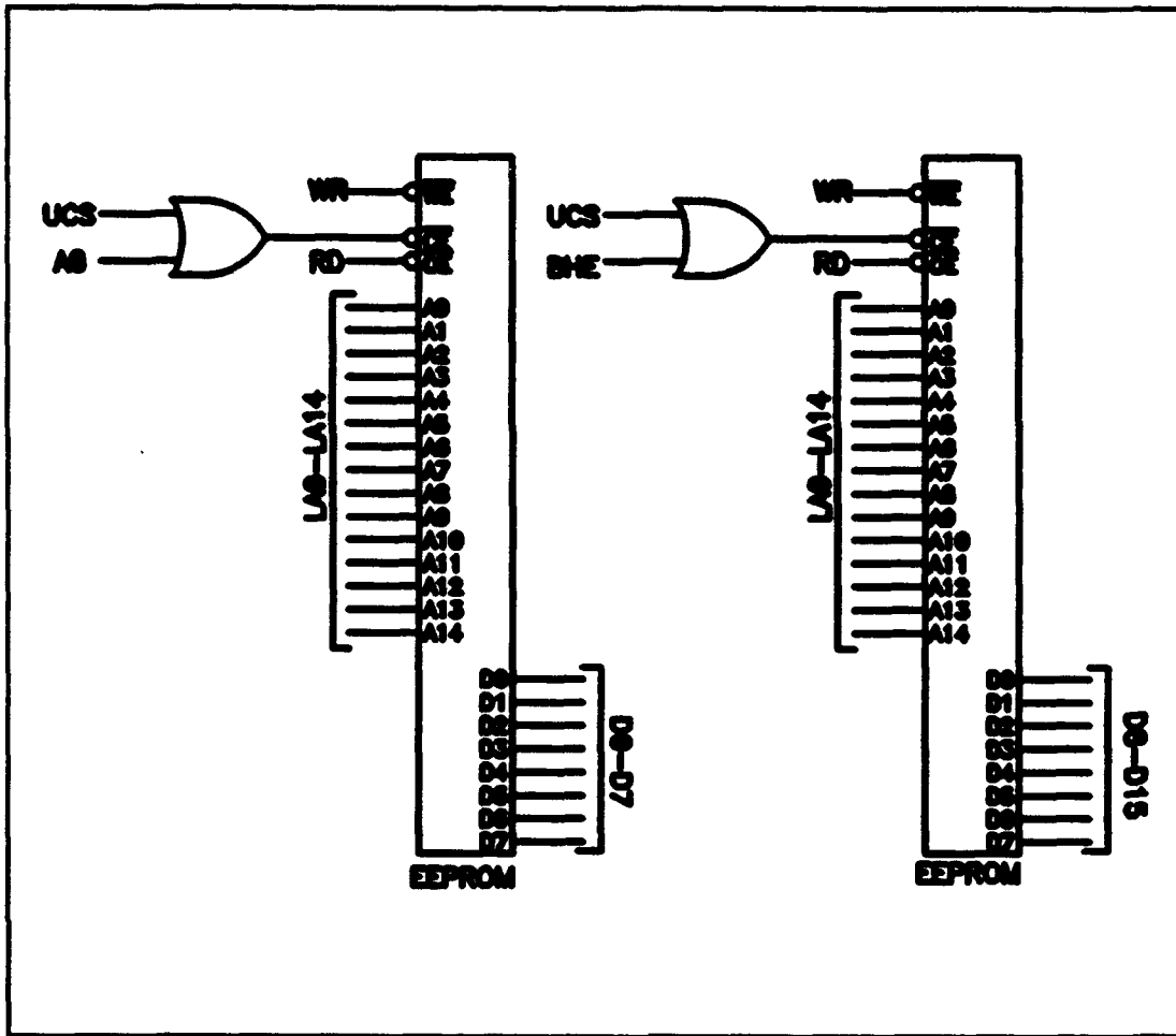
Figure 12 ROM Addressing
