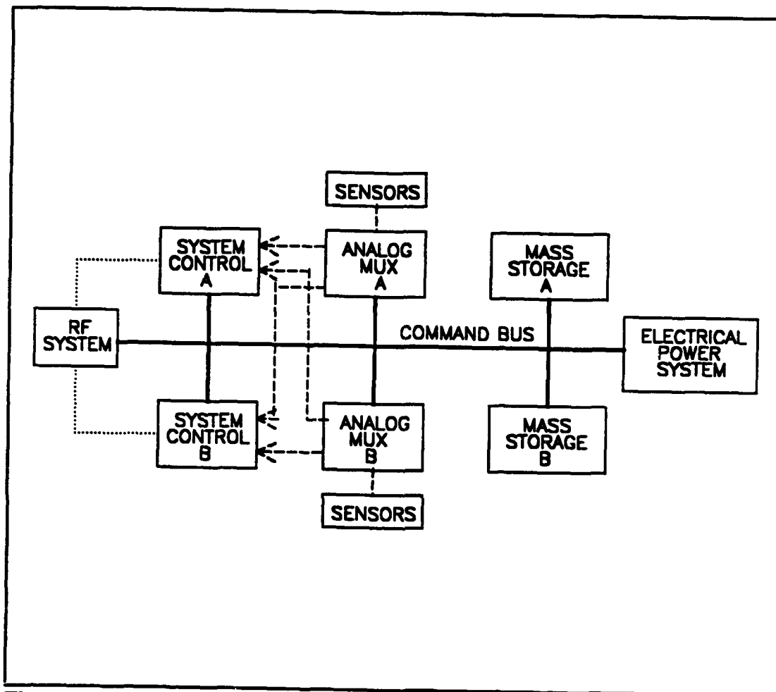
Figure 1 PANSAT Block Diagram
