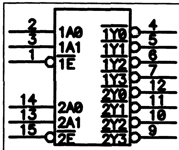
Figure 24 HCTS139MS
