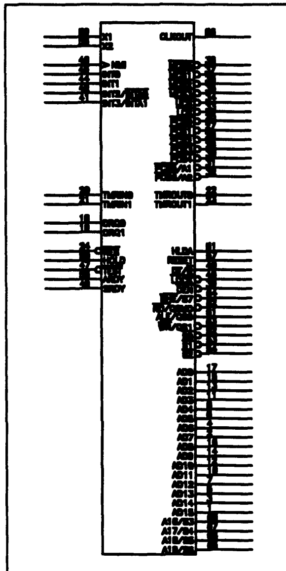
Figure 4 M80C186
