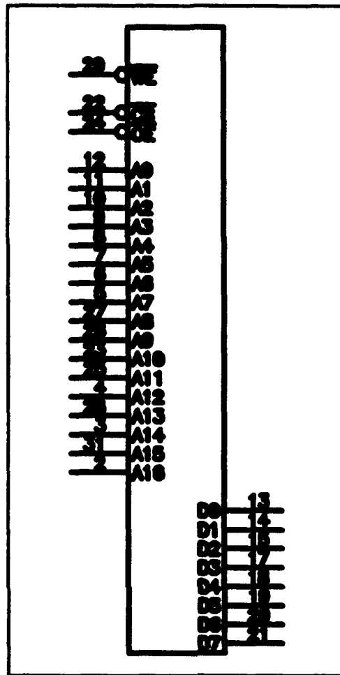
Figure 13 MSM8128JLMB-85
