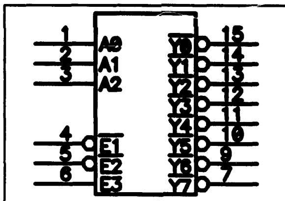
Figure 8 HCS138MS
