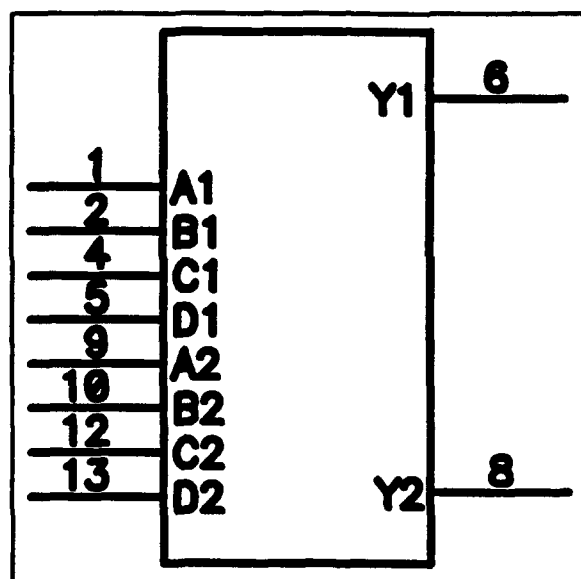
Figure 27 HCTS21MS
