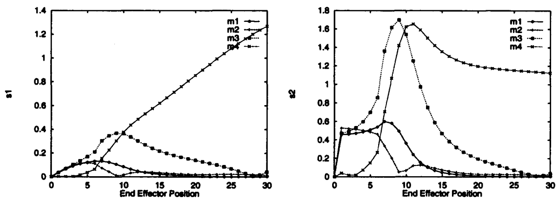
Figure 10: Sensitivities s_1 and s_2 to link masses for upper-actuated manipulator with 3 actuators
