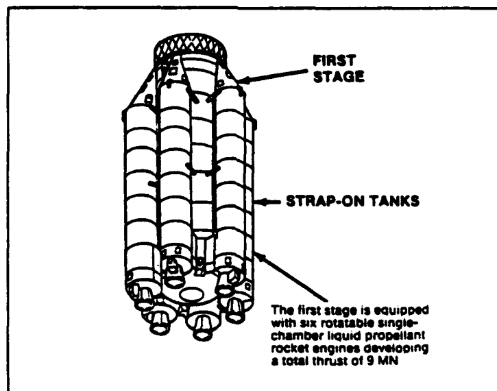
Figure 10. The Proton First Stage.
