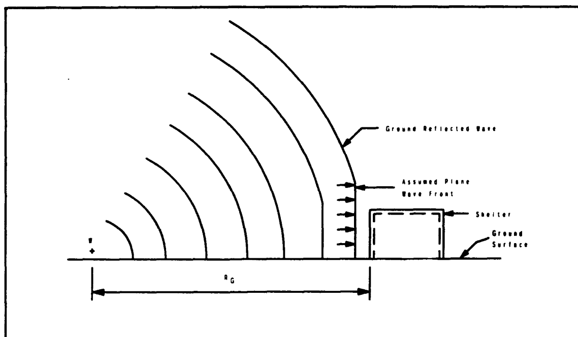
Figure 3.1 Surface Burst Blast Environment (TM5-855,1986)
