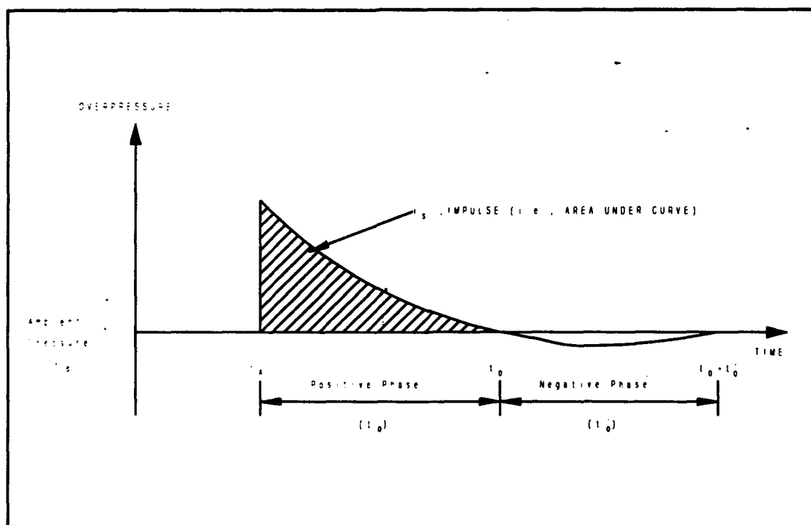
Figure 3.2 Typical Free-Field Pressure-Time History From a Conventional Weapon Detonation (TM5-855,1986)
