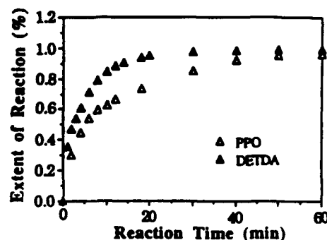
Fig.5 Extent of reaction measured via IR by following the disappearance of NCO group as a function of time for MDI/PPO reaction and MDI/DETDA reaction at 50°C
