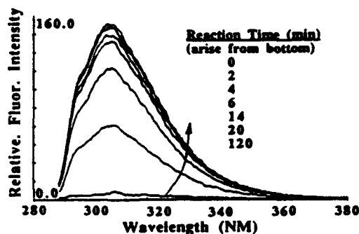
Fig.1 Fluorescence emission spectra for the reaction of MDI with excess 1-butanol in cyclohexane. Ex at 290 nm
