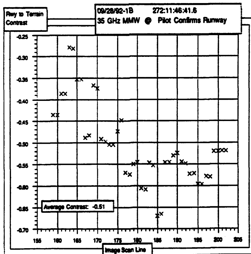
Figure 7-28. Contrast - September 28, 1992 - 1B (HTS at Pilot Confirms Runway)
