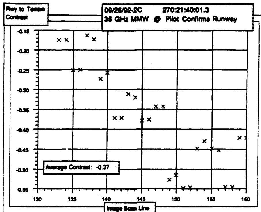
Figure 7-27. Contrast - September 26, 1992 - 2C (ORH at Pilot Confirms Runway)
