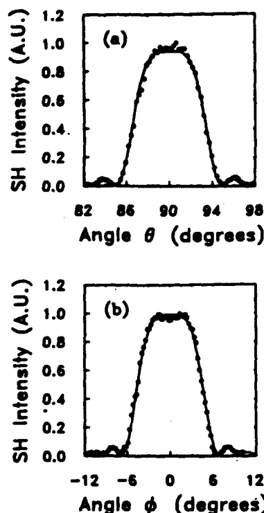
FIG. 2. External angular acceptances for second-harmonic generation of 1.064\text{ }\mu\text{m} radiation at the noncritical phase-matching temperature of 148.0 \pm 0.5^\circ\text{C} for rotation about (a) the Y axis ( \theta direction) and (b) the Z axis ( \phi direction). The FWHMs are 6.6^\circ and 9.1^\circ in the \theta and \phi directions, respectively.
