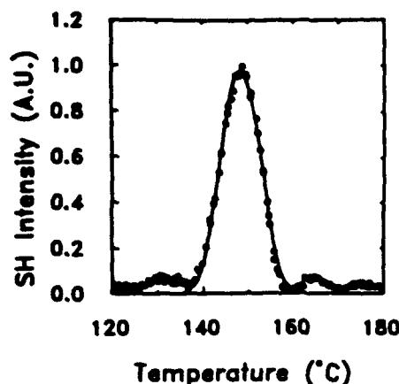
FIG. 1. Temperature tuning curve for noncritical phase matching at the fundamental wavelength of 1.064\text{ }\mu\text{m} in LBO. Noncritical phase matching occurs at 148.0 \pm 0.5^\circ\text{C} with a FWHM bandwidth of 10.1^\circ\text{C} .
