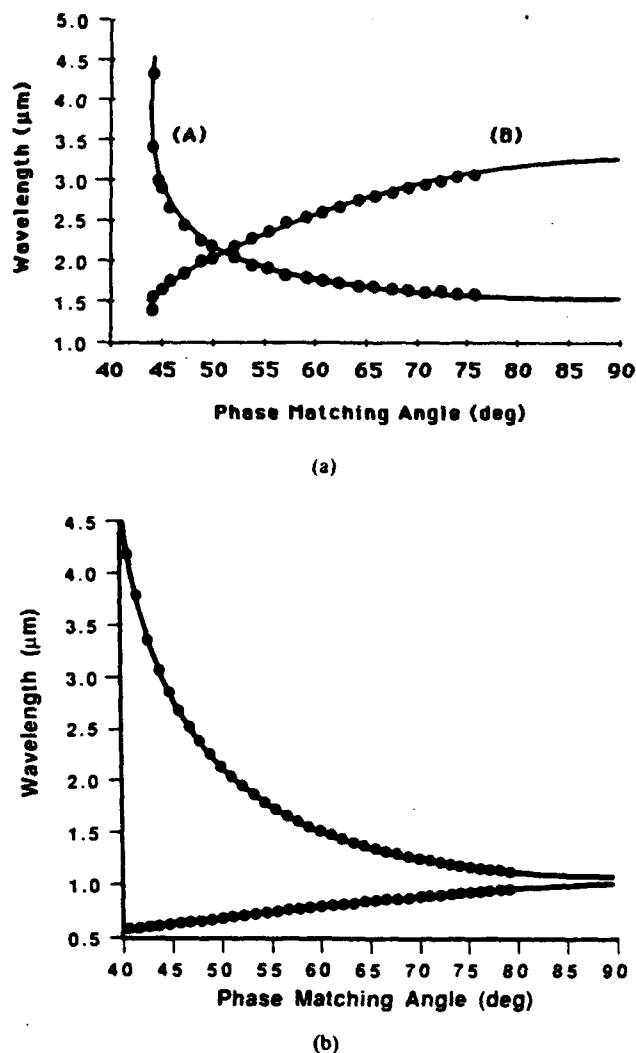
Fig. 4. Single-pass parametric generation tuning curves for KTP in the xy plane: (a) pumped at 1.053 \mu\text{m} and (b) at 526 nm. The tuning gap in (b) is from 1.007 to 1.103 \mu\text{m} and can be removed by going to o \sim 23^\circ plane. (Reprinted from [18]).
