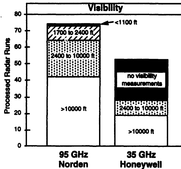
Figure 13b. MMW Test Data Matrix Sorted by Along-Path Visibility
