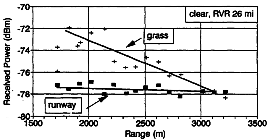
Figure 15b. 95 GHz Downrange Power Profile
