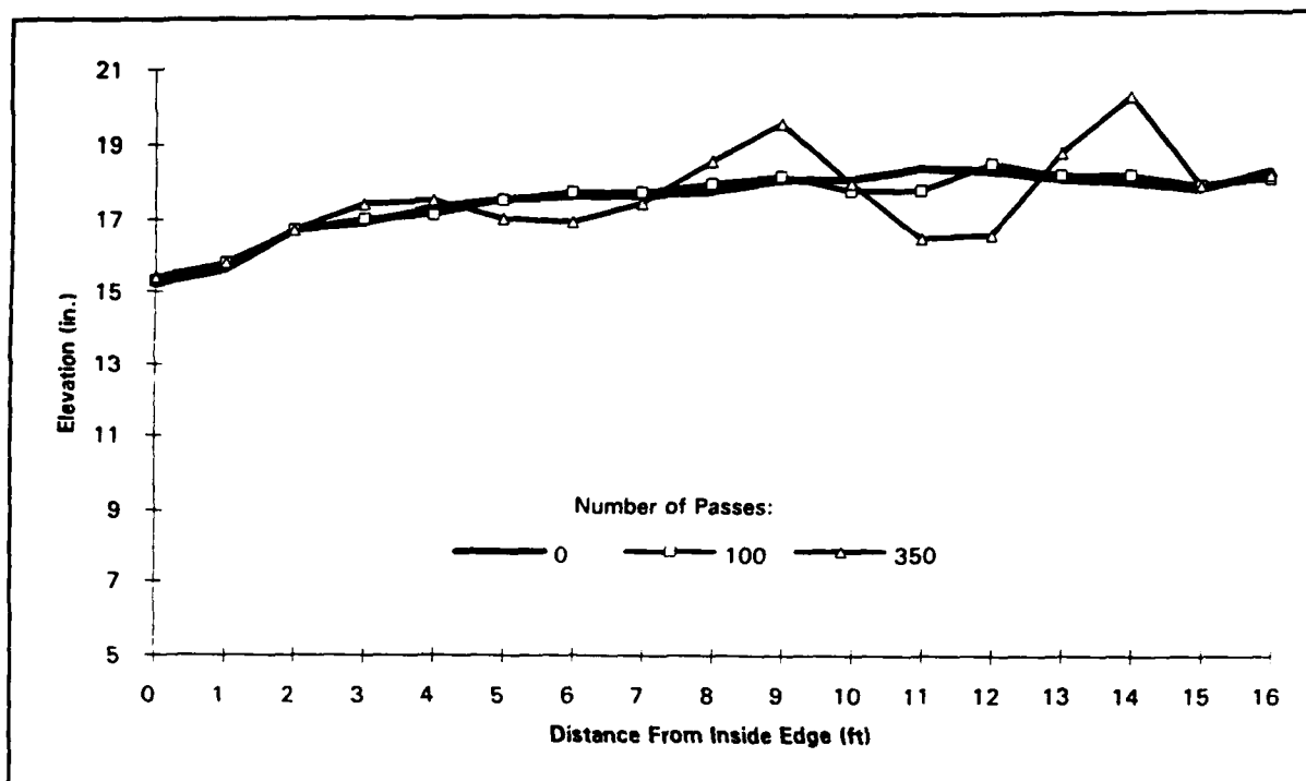
Figure 11. Section 2 (6-in. sand, 5-percent cement) cross sections (sta 0+43) (traffic terminated at 350 passes due to failure)
