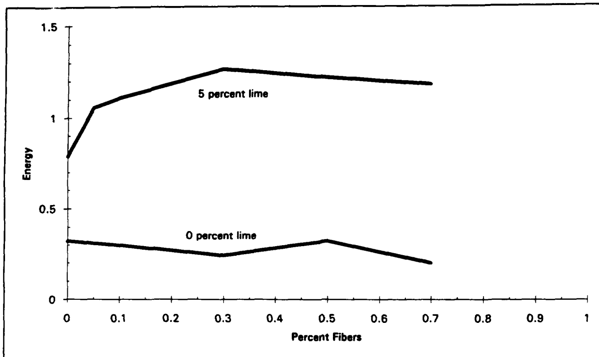
Figure 1. Energy versus percent fiber by weight of dry soil for clay (energy in ft-lb/in. 3 )
