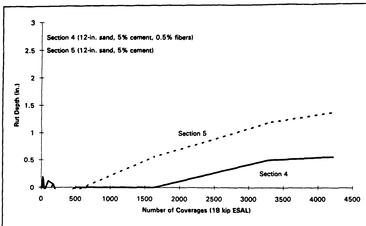
Figure 27. Measured rut depth progression, sections 4 and 5
