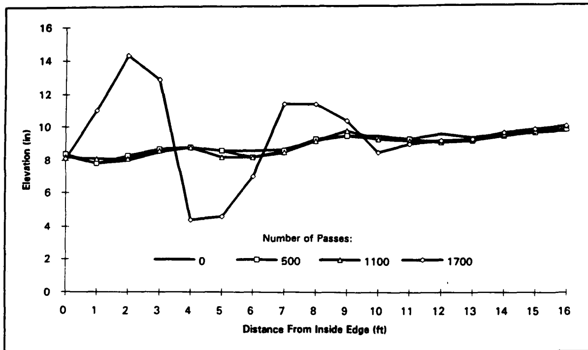
Figure 21. Section 12 (6-in. clay, 5-percent lime, 0.1-percent fibers) cross sections (sta 1 + 39) (traffic terminated at 1,700 passes due to failure)
