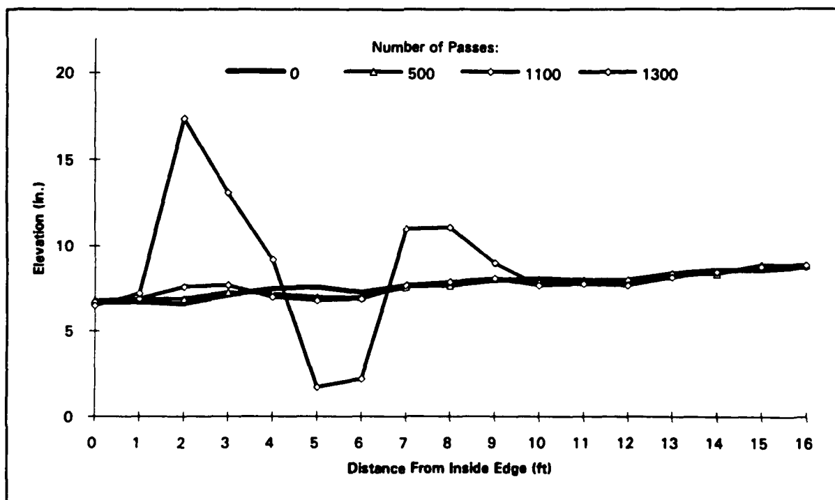
Figure 22. Section 13 (6-in. clay, 5-percent lime) cross sections (sta 1 + 70) (traffic terminated at 1,300 passes due to failure)
