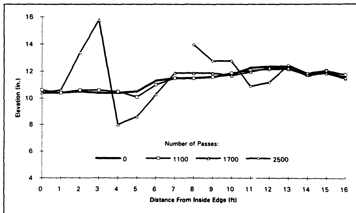
Figure 20. Section 11 (6-in. clay, 5-percent lime, 0.3-percent fibers) cross sections (sta 1+08) (traffic terminated at 2,500 passes due to failure, inside wheel path failed at 1,900 passes)
