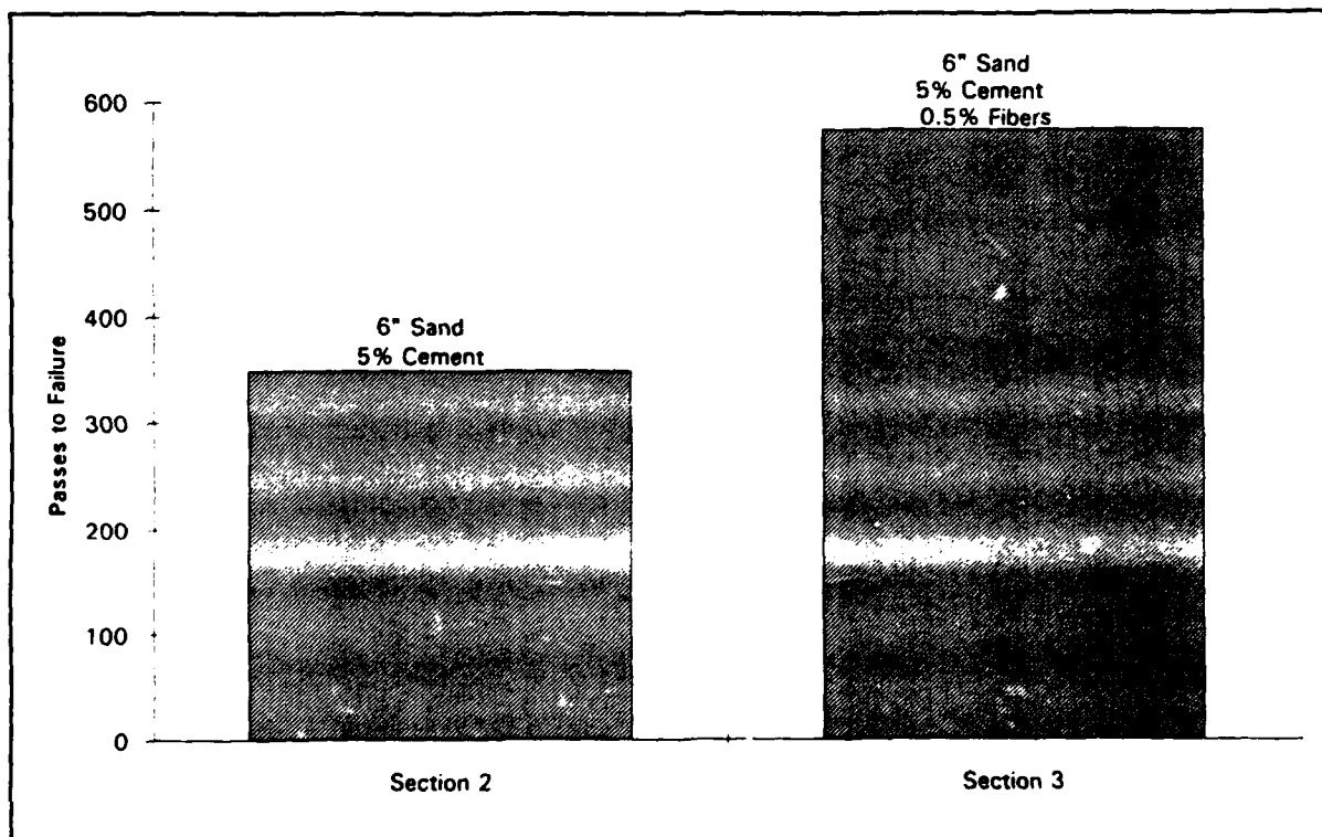
Figure 25. Comparison of sections 2 and 3
