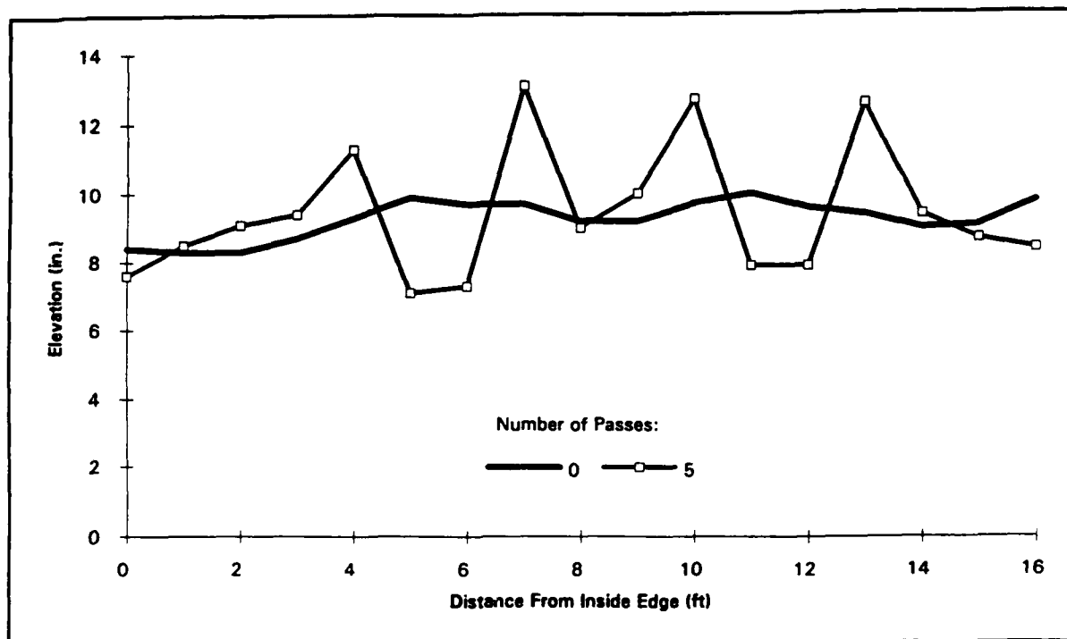
Figure 17. Section 8 (12-in. clay) cross sections (sta 0 + 14) (traffic terminated at 5 passes due to failure)
