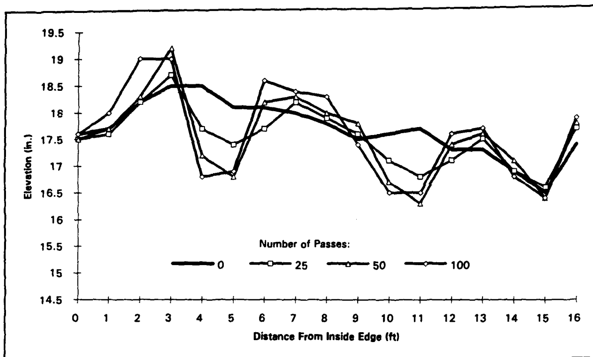
Figure 15. Section 6 (12-in. sand, 0.5-percent fibers) cross sections (sta 1 + 67) (traffic terminated at 100 passes due to failure)
