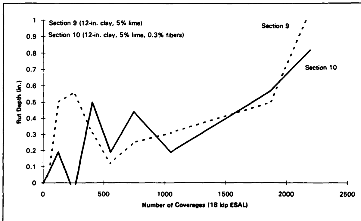
Figure 29. Measured rut depth progression, sections 9 and 10
