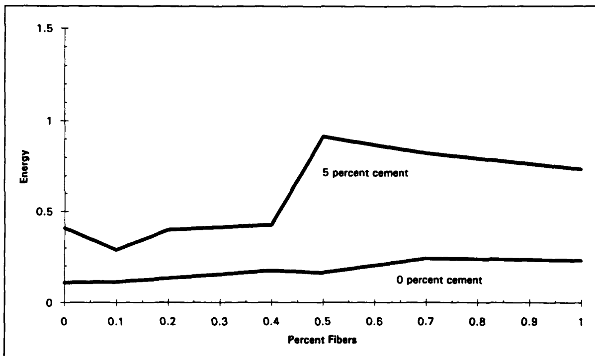
Figure 2. Energy versus percent fiber by weight of dry soil for sand (energy in ft-lb/in. 3 )
