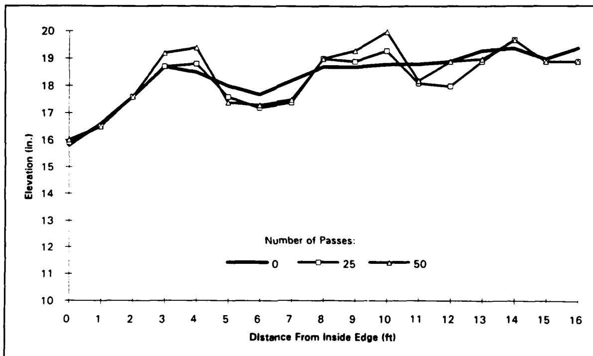
Figure 10. Section 1 (6-in. sand, 0.5-percent fiber) cross sections (sta 0 + 13) (traffic terminated at 50 passes due to failure)
