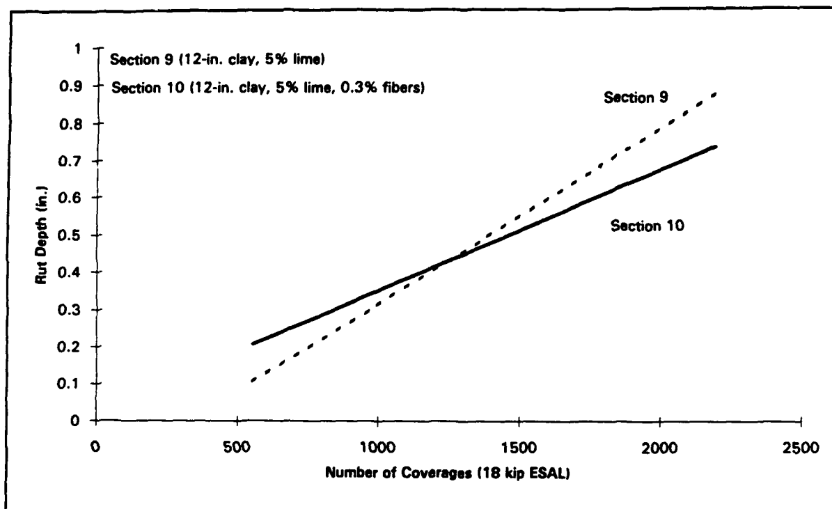
Figure 30. Lines fitted to data for sections 9 and 10
