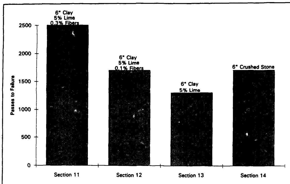
Figure 26. Comparison of sections 11, 12, 13, and 14
