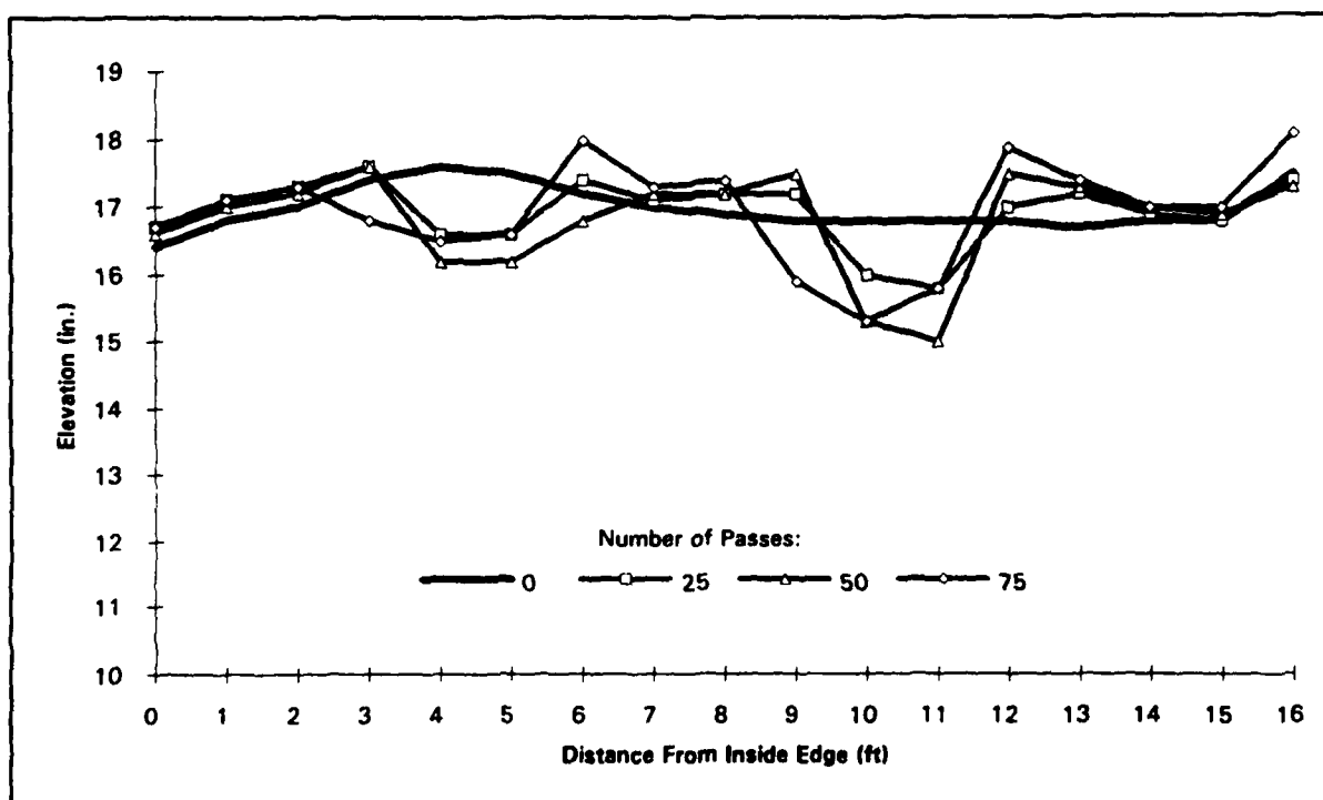
Figure 16. Section 7 (12-in. sand) cross sections (sta 1 + 99) (traffic terminated at 75 passes due to failure)
