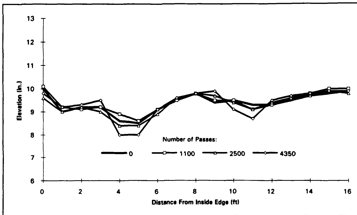
Figure 18. Section 9 (12-in. clay, 5-percent lime) cross sections (sta 0 + 46) (traffic terminated at 4,350 passes due to termination of testing)
