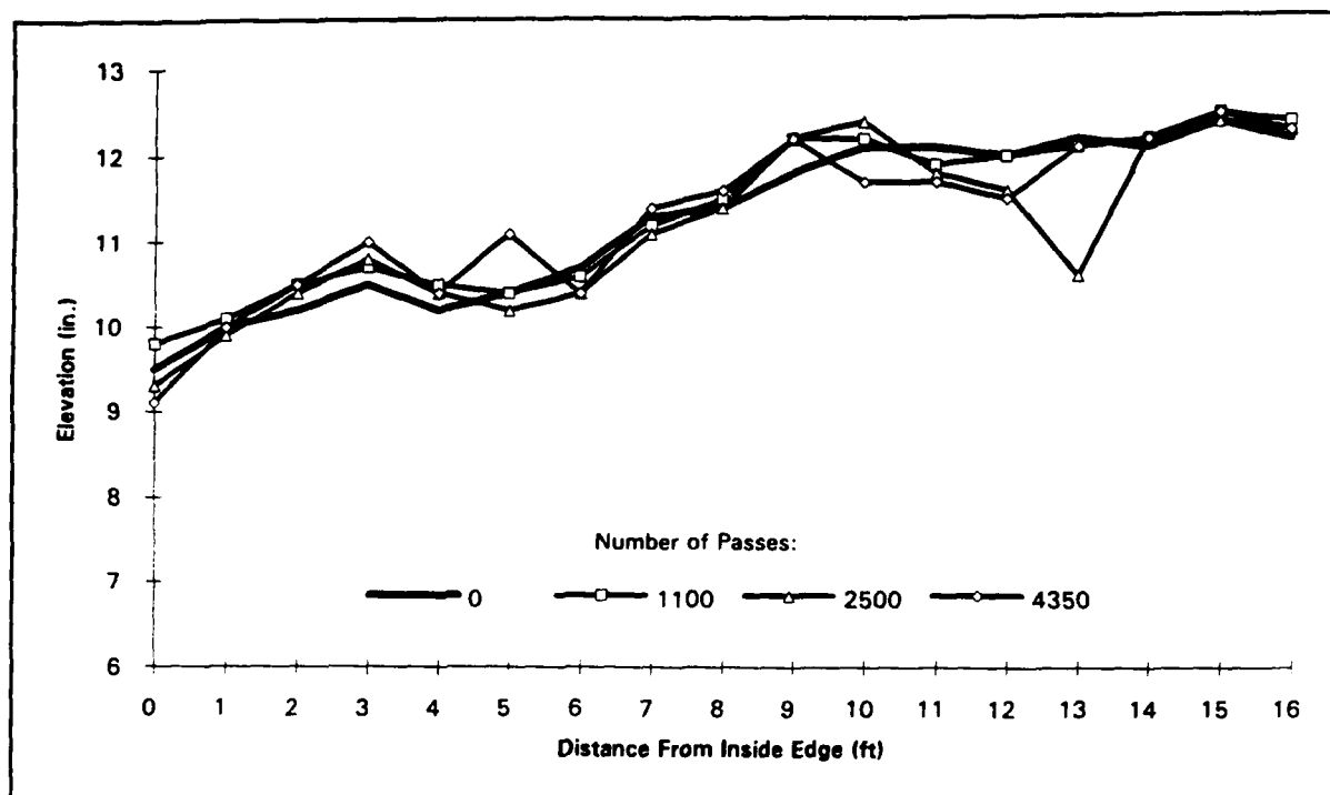
Figure 19. Section 10 (12-in. clay, 5-percent lime, 0.3-percent fibers) cross sections (sta 0+76 (traffic terminated at 4,350 passes due to termination of testing))
