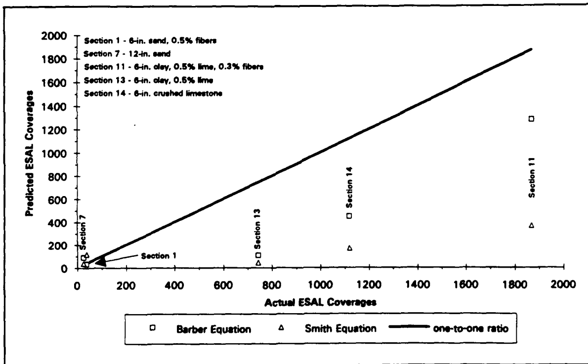
Figure 32. Comparison of actual to predicted coverages (ratio of measured surface CBR to subgrade CBR of less than 10)
