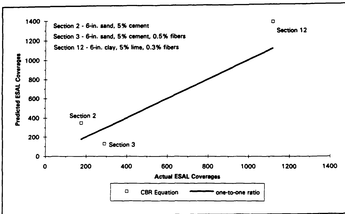
Figure 31. Comparison of actual to predicted coverages (ratio of measured surface CBR to subgrade CBR of 10 or greater)
