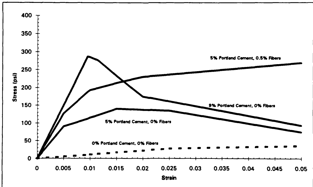
Figure 4. Stress-strain curves for sand
