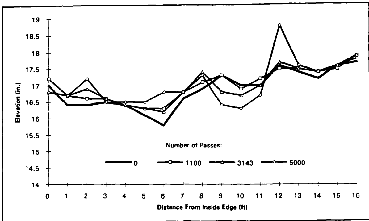
Figure 13: Section 4 (12-in. sand, 5-percent cement, 0.5-percent fibers) cross sections (sta 1 + 05) (traffic terminated at 5,000 passes due to complete application of design traffic)
