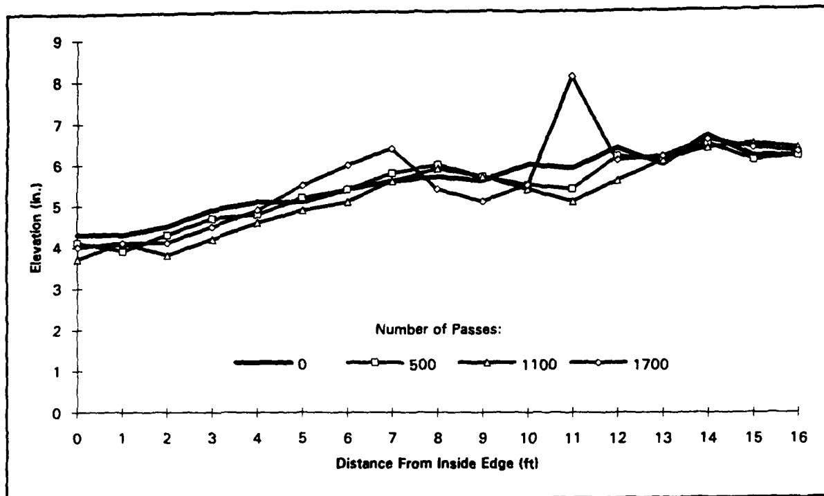
Figure 23. Section 14 (6-in. crushed limestone) cross sections (sta 2 + 00) (traffic terminated at 1,700 passes due to failure)
