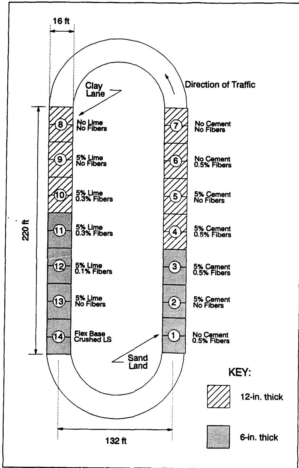
Figure 5. Layout of test track
