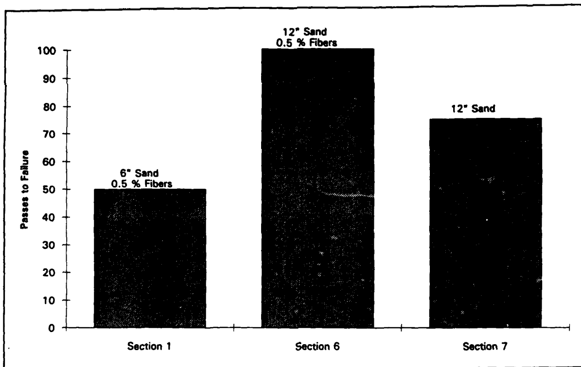
Figure 24. Comparison of sections 1, 6, and 7
