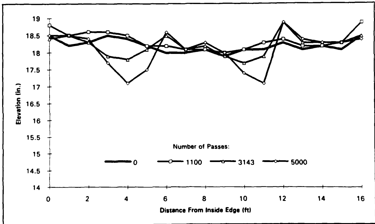
Figure 14: Section 5 (12-in. sand, 5-percent cement) cross sections (sta 1 + 36) (traffic terminated at 5,000 passes due to complete application of design traffic and impending failure)
