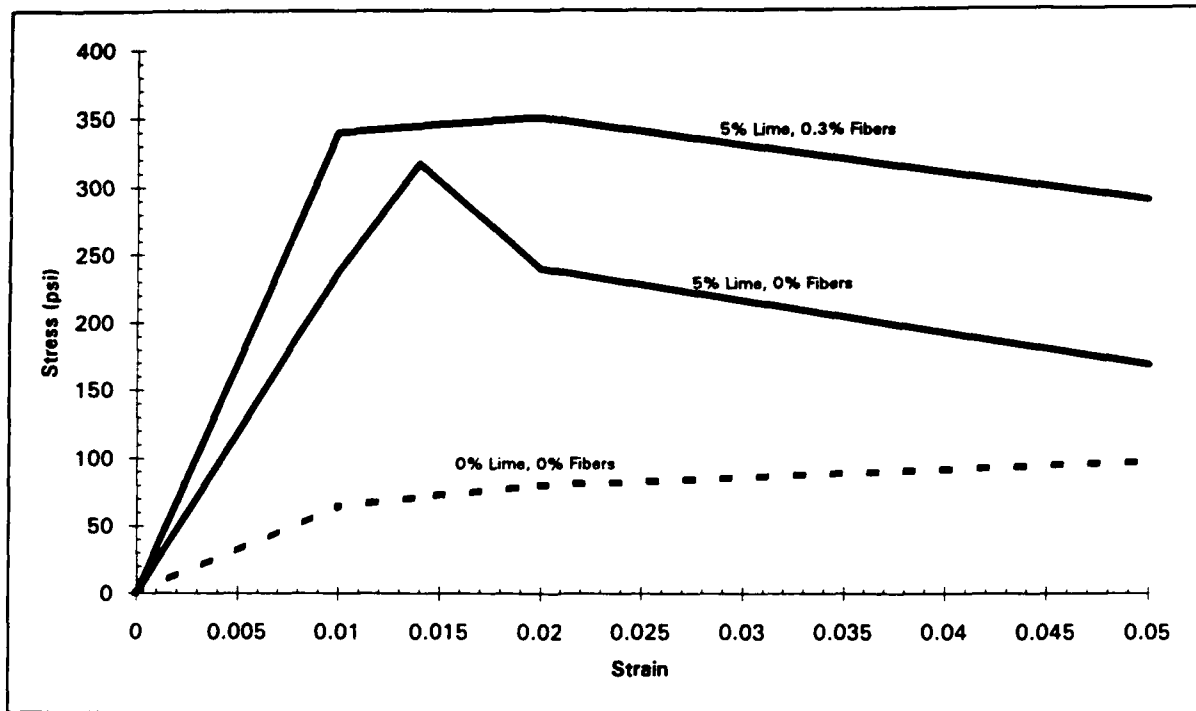
Figure 3. Stress-strain curves for clay
