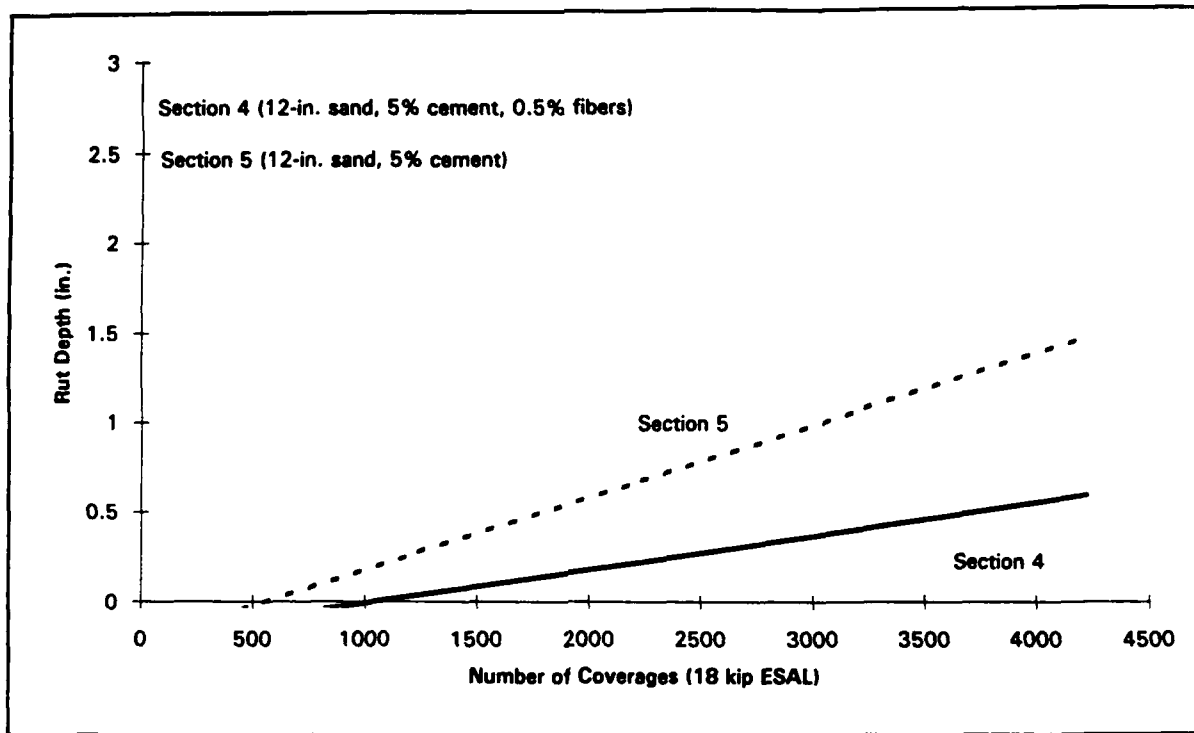
Figure 28. Lines fitted to data for sections 4 and 5
