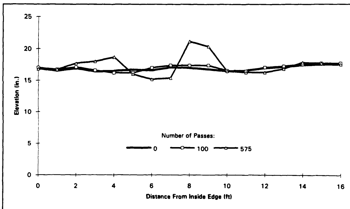
Figure 12. Section 3 (6-in. sand, 5-percent cement, 0.5-percent fibers) cross sections (sta 0+74) (traffic terminated at 575 passes due to failure)
