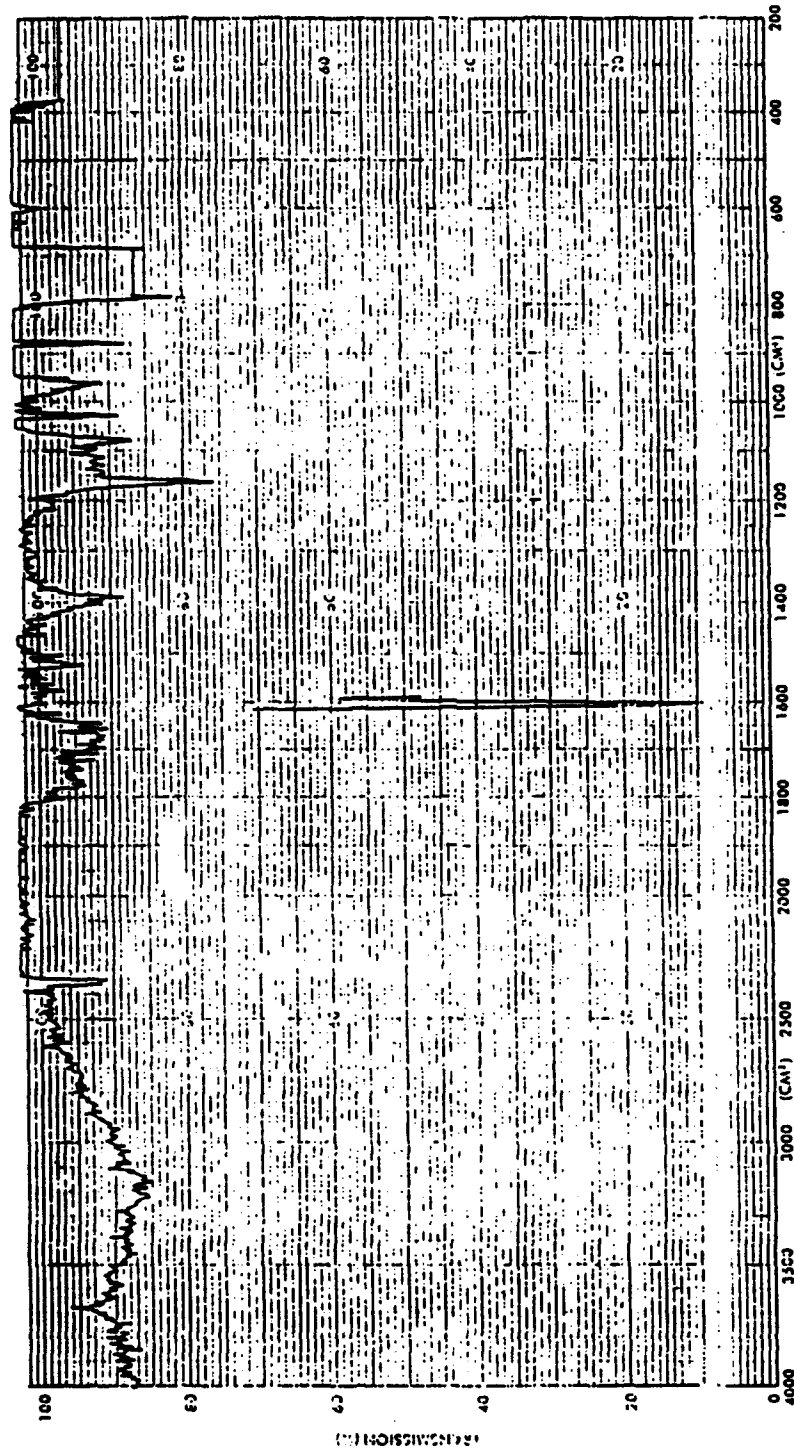
Figure 4.9 IR (CDCl 3 ) trans-Di(3-Furyl)ethylene.
