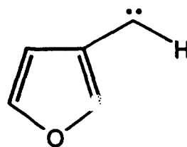
1.2 3-furylmethylene
