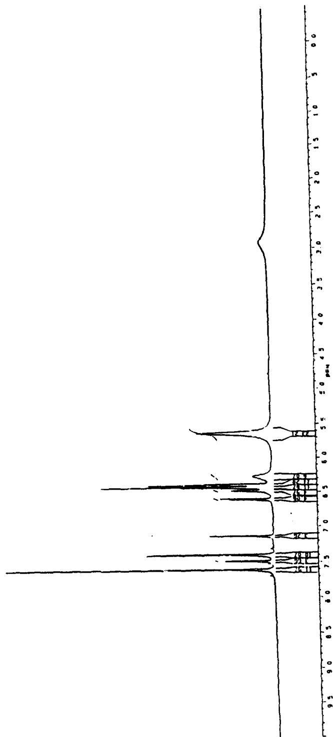
Figure 4.2 ^1\text{H} NMR ( \text{CDCl}_3 , 250 MHz) 2-Furylhydrazone.
