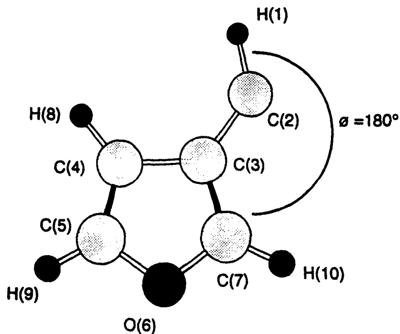
Figure 2.14 Chem3D Rendering of Triplet 3-Furylmethylene ( \theta = 180^\circ ) calculated using MP2/6-31G*.
