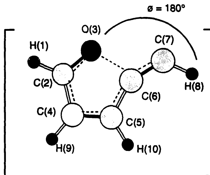
Figure 2.9 Chem3D Rendering of the Transition State [2-Furylmethylene \rightarrow cis-2-penten-4-ynal] ( \theta = 180 ) calculated using MP2/6-31G*.
