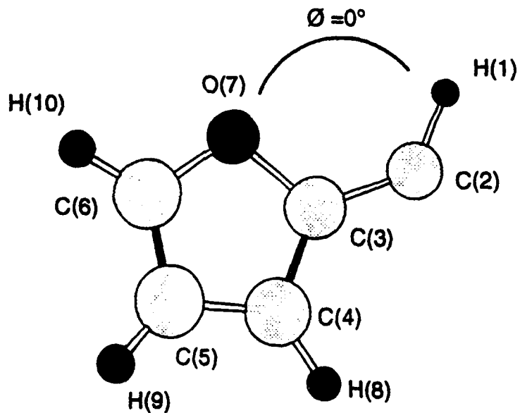
Figure 2.8 Chem3D Rendering of Triplet 2-Furylmethylene ( \varnothing = 0^\circ ) calculated using UHF/6-31G*.
