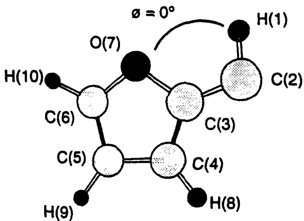
Figure 2.6 Chem3D Rendering of Singlet 2-Furylmethylene ( \theta = 0^\circ ) calculated using HF/6-31G*.
