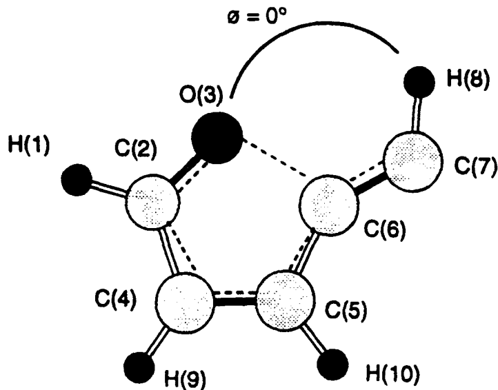
Figure 2.10 Chem3D Rendering of Transition State [2-Furylmethylene \rightarrow cis-2-penten-4-ynal] ( \vartheta = 0^\circ ) calculated using HF/6-31G*.
