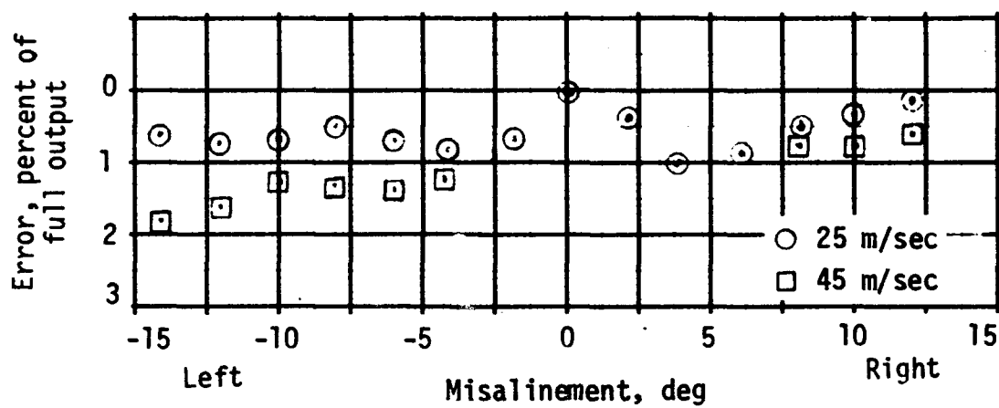
Figure 11.- Variation of anemometer output with misalignment.
