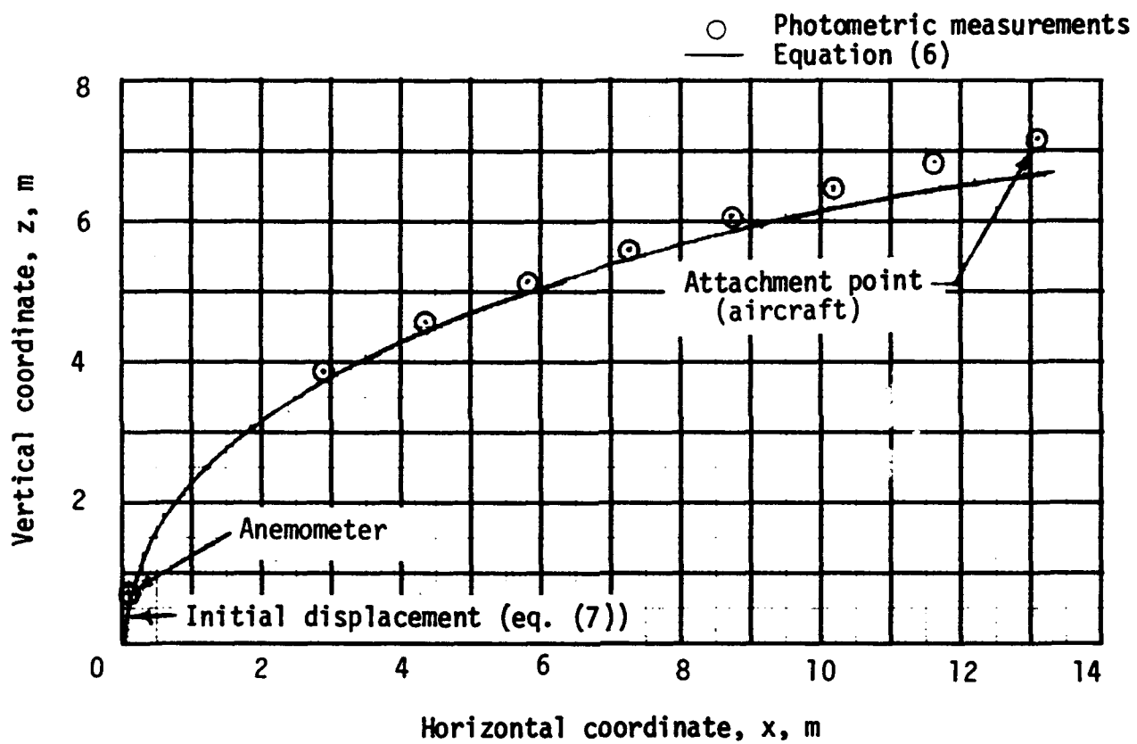
Figure 14.- Shape of anemometer cable when operating at dynamic pressure of 1.93 kPa with 17 m of cable deployed.
