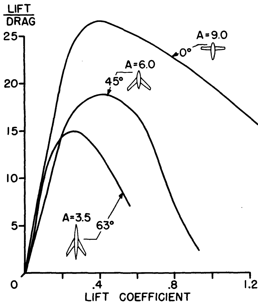
Figure 8. - The value of lift-drag ratio as a function of lift coefficient for three wings having different values of sweepback and aspect ratio.
