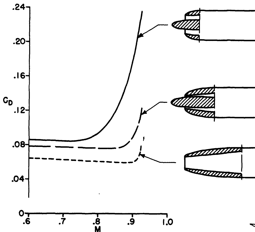
Figure 10. - Effect of Mach number on the external drag characteristics of three nose inlets.
