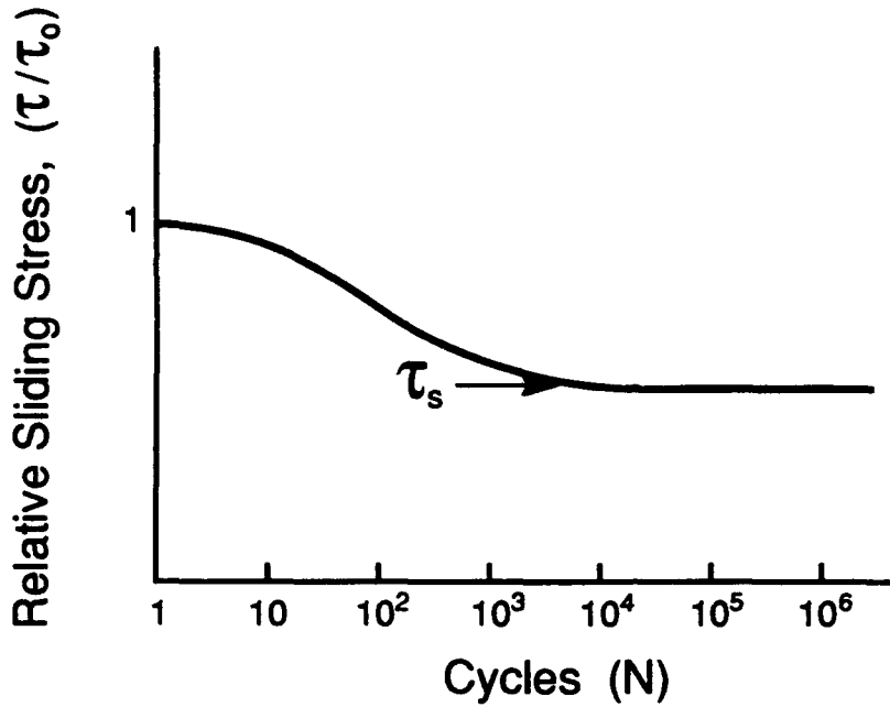
Reduction In Interface Sliding Resistance During Fatigue
