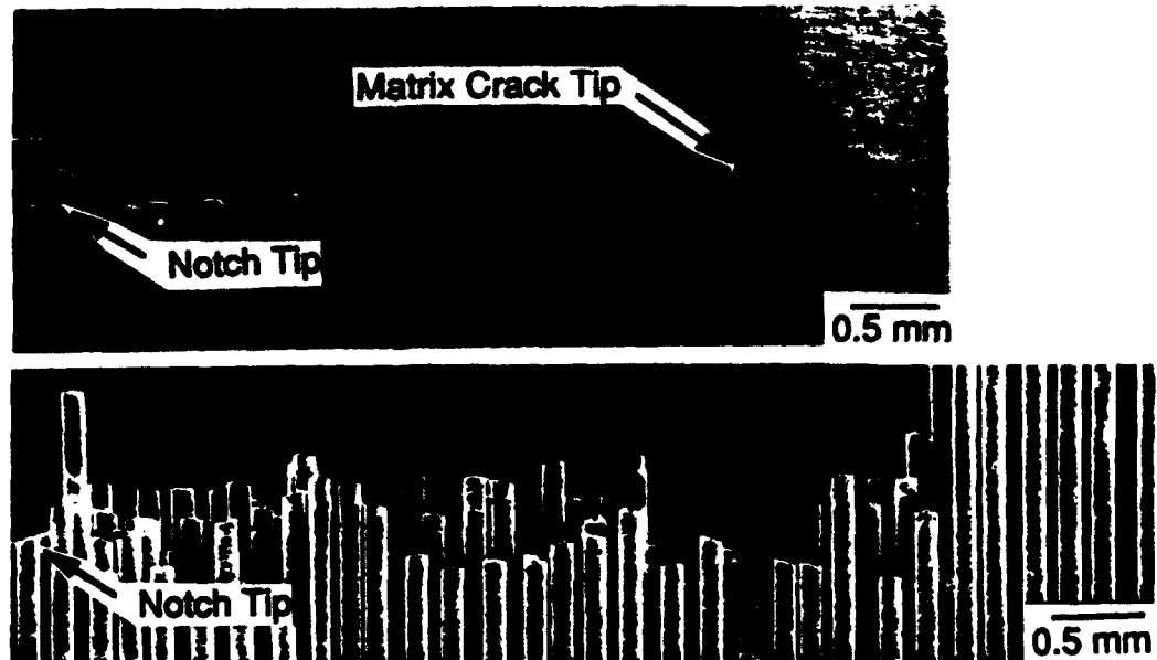
Fig. 8. Comparison of matrix crack and underlying fibers for test conducted at \Delta\sigma_c = 400 MPa, R = 0.1 and 2a_0 = 9 mm. Note the absence of intact fibers in the crack wake and the extent of fiber failure ahead of the crack tip.
