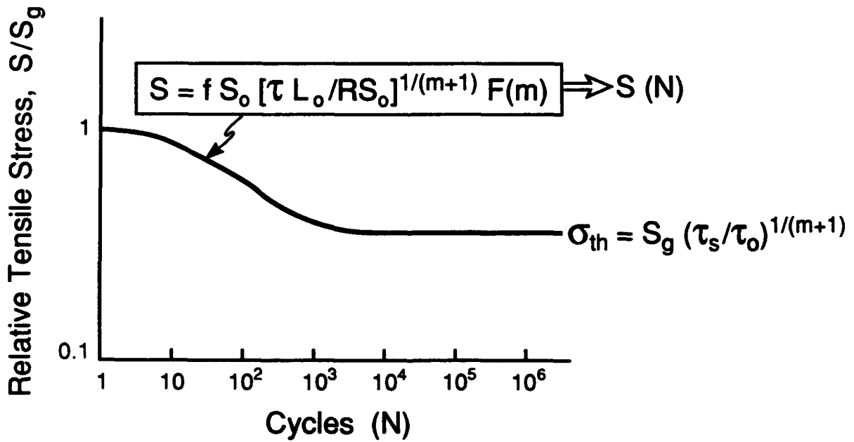
Reduction in UTS Caused By Interface Degradation
