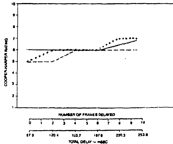
Figure 6.28 Effects of manual display lags ( , , ) of flight manoeuvres (Median of 4 subjects, adapted from ref. 1).
