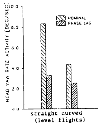
Figure 6.14 Yaw-axis head motion velocities (standard deviation) in the flight path estimation task with and without an exponential display lag of e^{-t/0.5s} (adapted from ref. 1).
