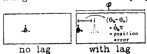
Figure 6.1 Diagrammatic illustration of the effect of lag between head movement and image captured by a head-slaved camera (The effect is similar to that of display lags, adapted from ref. 6).
