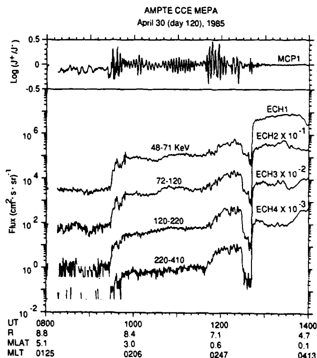
Fig. 15. Ion data from the MEPA instrument on CCE for the day 120 event. In the upper panel is the ratio (referred to as anisotropy in the text) of MCP1 counts of the downward moving ions to those of the duskward moving ions at 90^\circ pitch angle. The lower panel shows 24-s (four spins) averages of ion fluxes measured by the ion head of MEPA.
