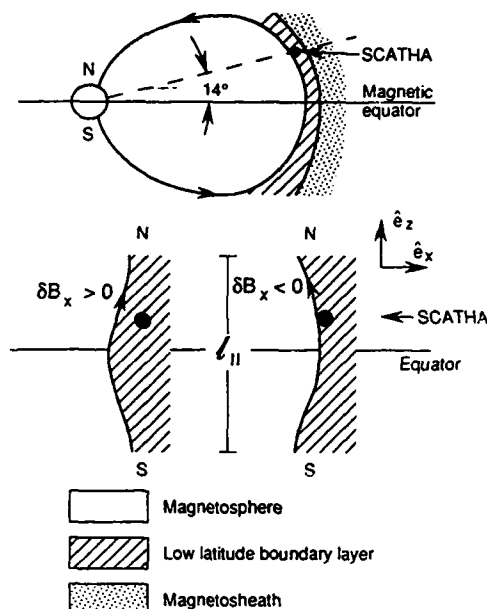
Fig. 10. (Top) A schematic for the satellite location with respect to the magnetic equator and the LLBL and (bottom) an enlarged view of the boundary layer at two epochs of \delta B_x .
