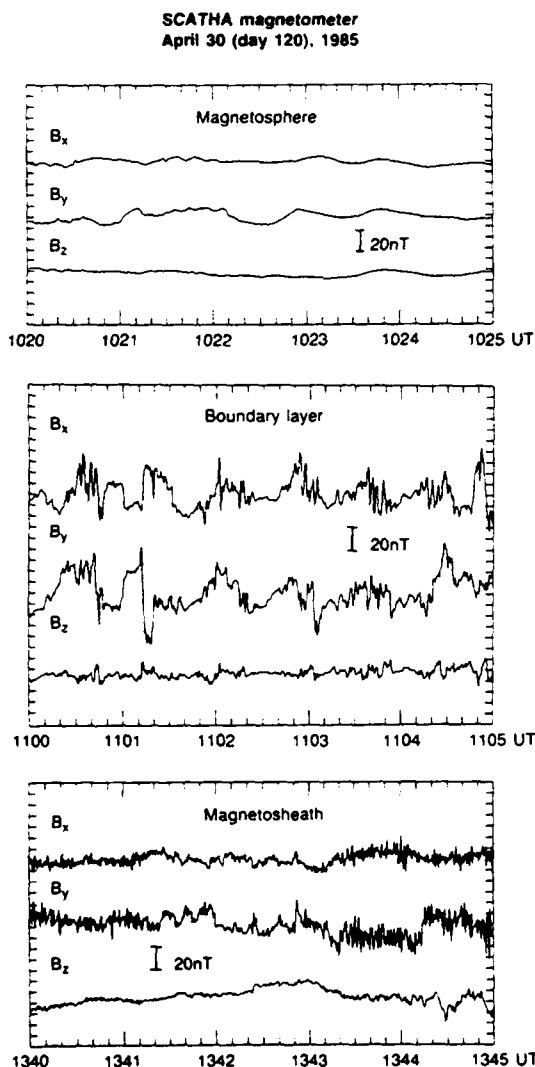
Fig. 7. High-time-resolution (0.25 s) magnetic field data from different regions near the magnetopause. The field is rotated into local field-aligned coordinates, in which \hat{e}_z (parallel component) is along the direction of the average magnetic field for the time interval displayed, \hat{e}_y (azimuthal component) is in the direction of \hat{e}_z \times \mathbf{r} , where \mathbf{r} is the position vector of the spacecraft with respect to the center of the Earth, and \hat{e}_x (radial component) = \hat{e}_y \times \hat{e}_z .
