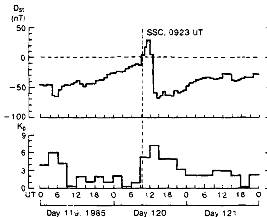
Fig. 1. Geomagnetic indices (top) Dst and (bottom) Kp at the time of the storm sudden commencement on April 30 (day 120), 1985.
