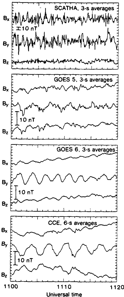
Fig. 18. Simultaneous observations of magnetic field oscillations in the boundary layer (SCATHA) and in the magnetosphere (GOES 5, GOES 6, and CCE). Field components are all given in the local mean-field-aligned coordinate described in the text.
