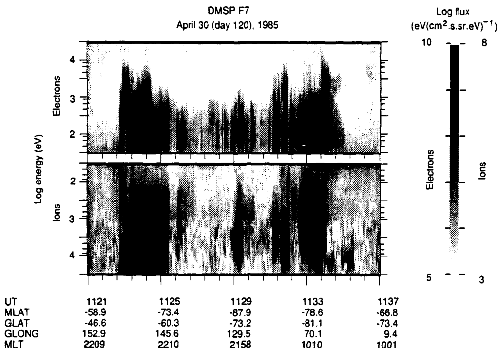
Fig. 3. DMSP F7 precipitation particle data suggesting northward IMF.
