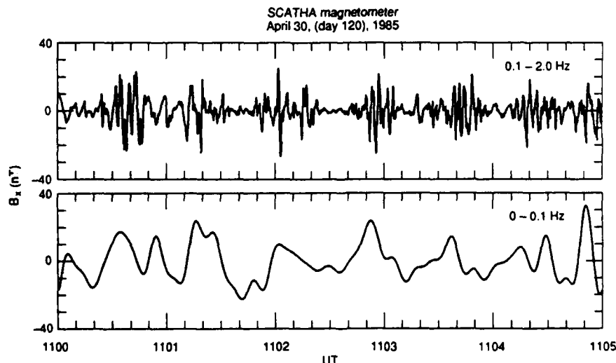
Fig. 12. High- and low-pass-filtered data showing an envelope structure of higher-frequency oscillations and its relationship to the phase of a lower-frequency oscillation.
