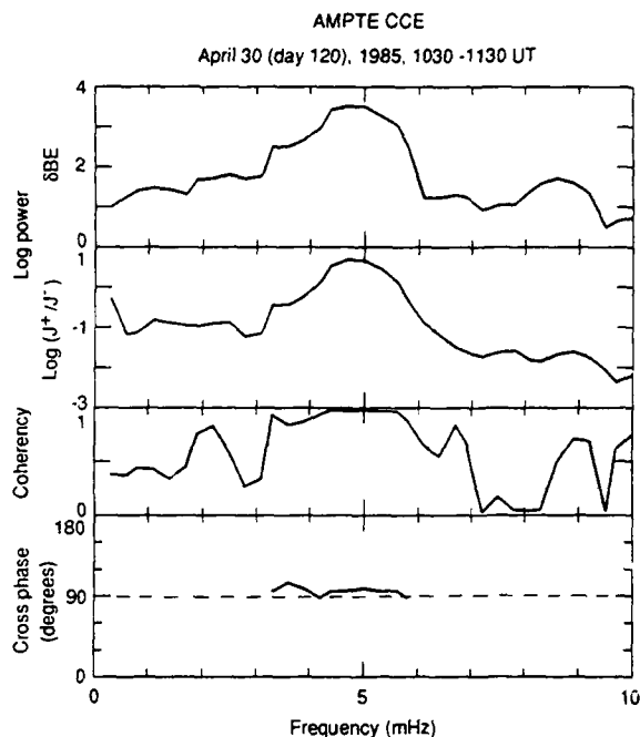
Fig. 17. Cross spectral analysis of the particle flux and magnetic field pulsations shown in Figure 16. The cross phase is shown only for frequency components with high ( > 0.8 ) coherency.
