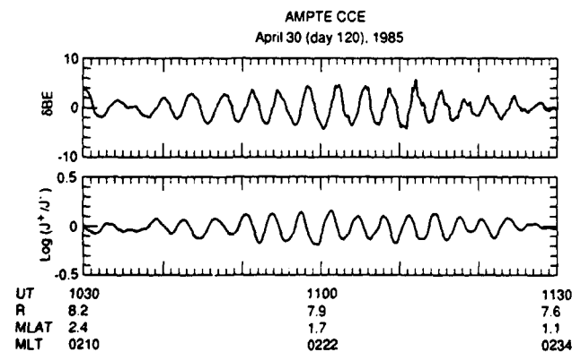
Fig. 16. Comparison of the (bottom) ion flux anisotropy oscillation from Figure 15 and the (top) azimuthal magnetic field for the same time interval.
