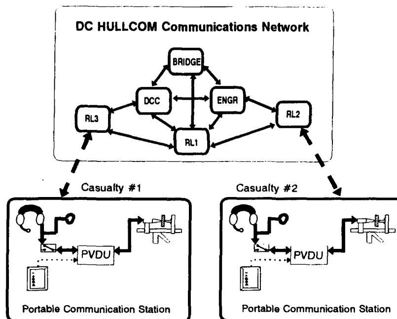
Fig. 13 — Portable communications station interface
