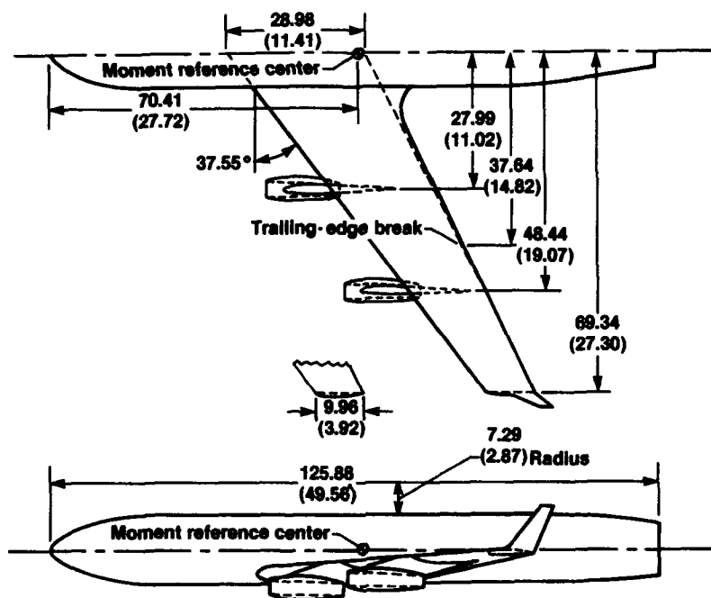
Figure 6. General layout of high-speed model. Dimensions are in centimeters (inches).
