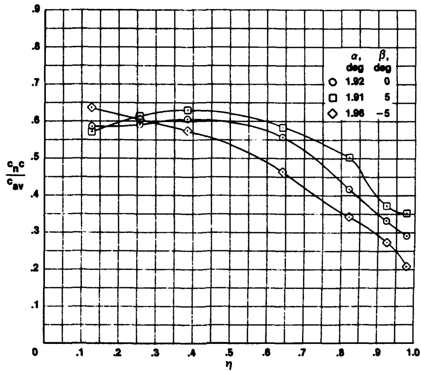
Figure 14. Variation of full-span model right wing panel load distributions with winglets for several angles of sideslip at a selected angle of attack. M_\infty = 0.78 ; q_\infty = 40.7 \text{ kPa} ( 850 \text{ lb/ft}^2 ).
